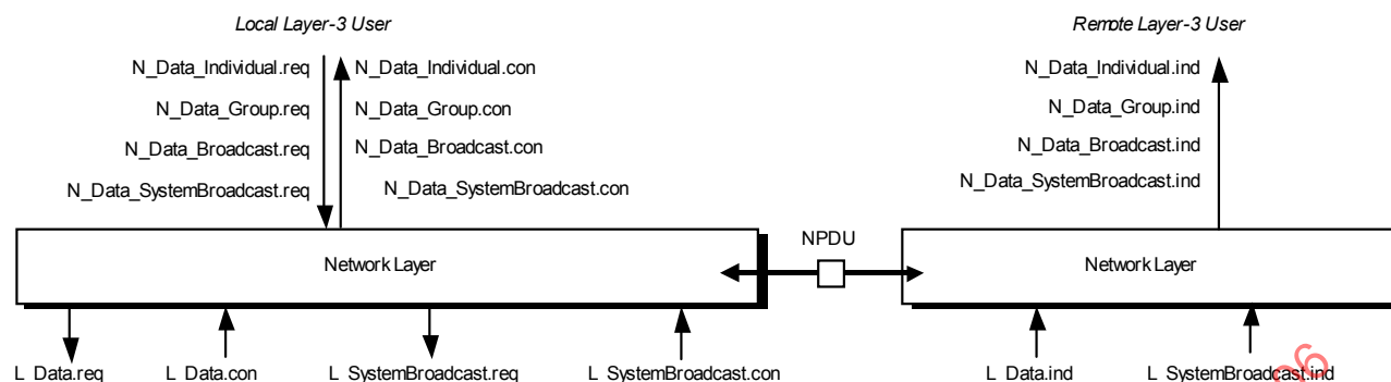
Figure 7 – Interaction of the network layer (not for bridges or routers)
