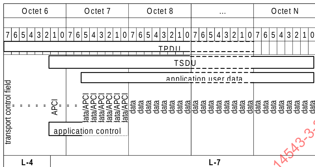
Figure 11 – Format of the TPDU (Example)
