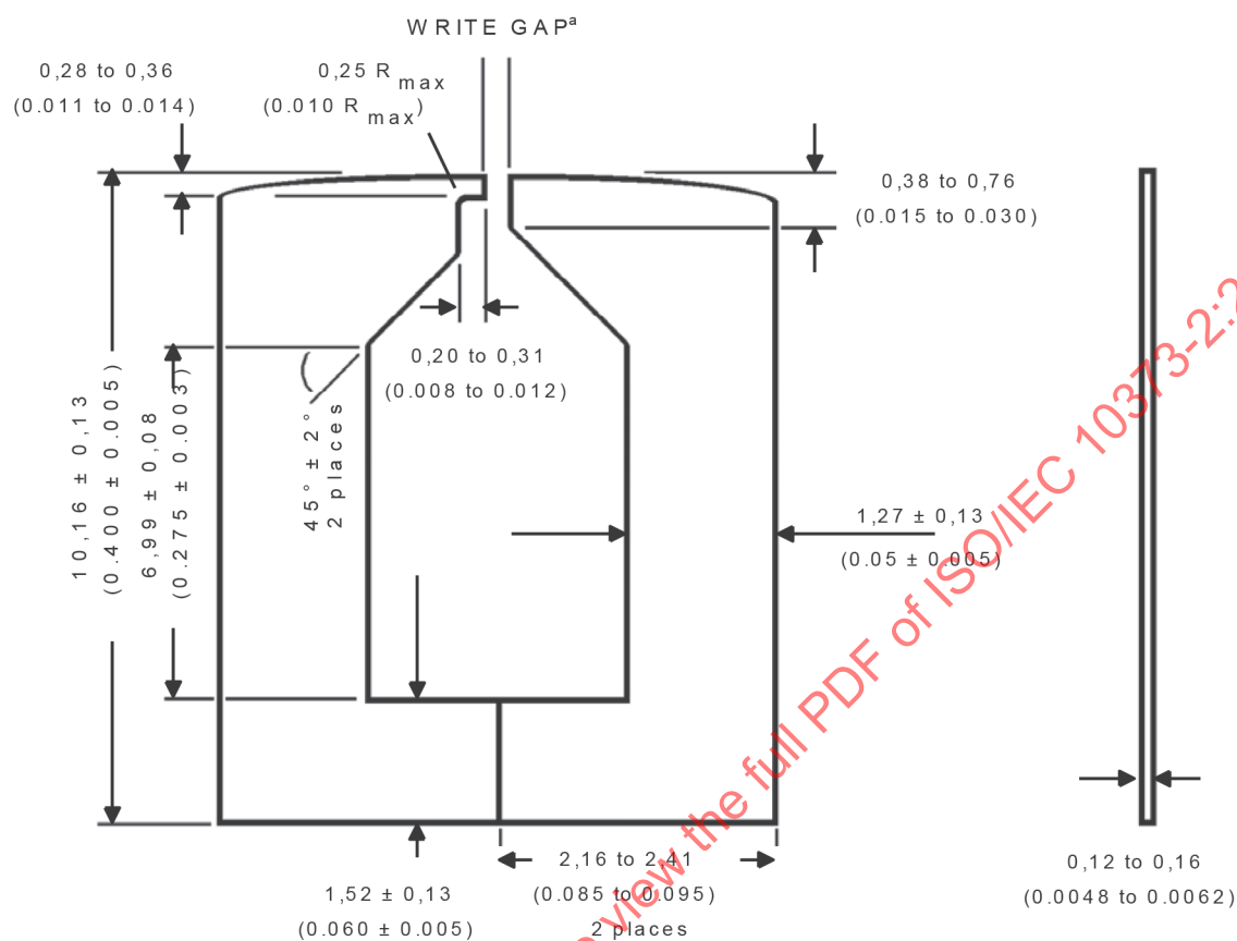
Figure 12 — Test write head laminations (dimensions in mm (inch), not to scale)
