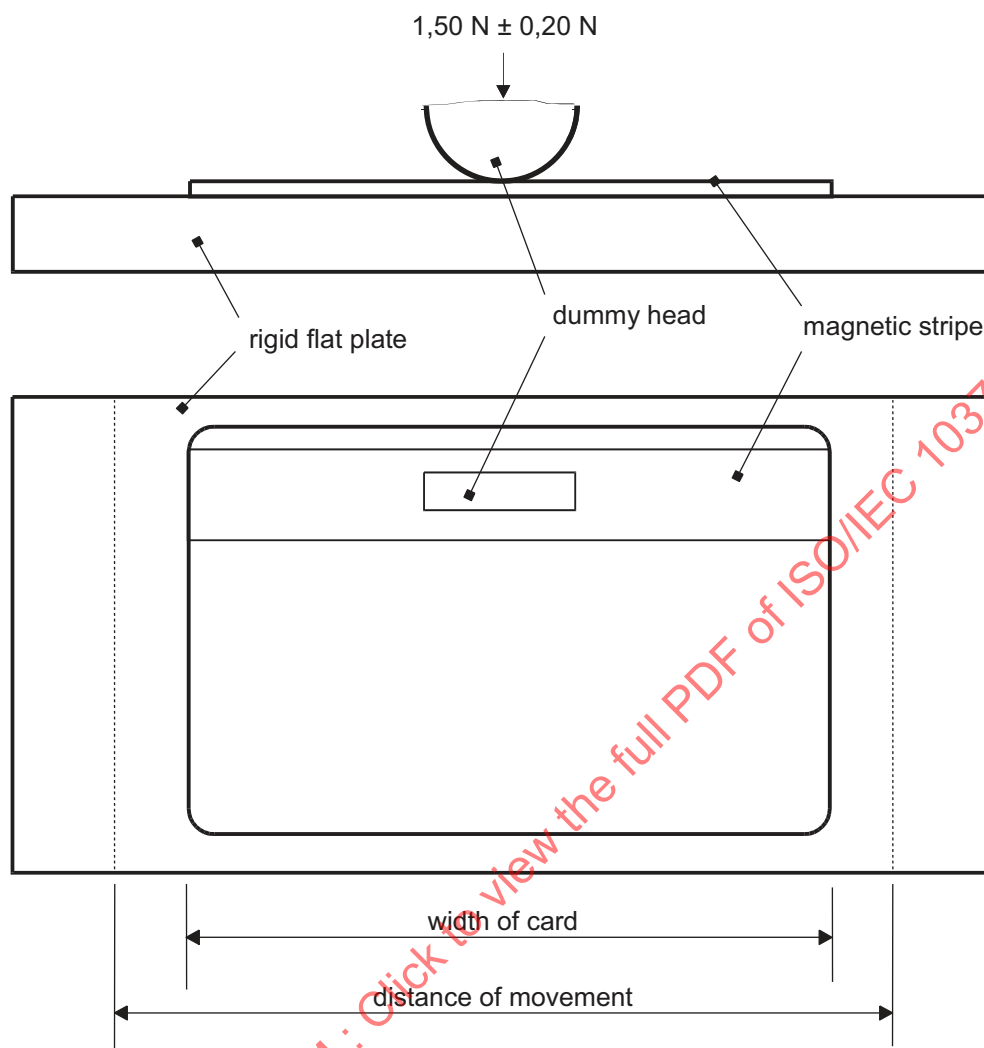
Figure 11 — Dummy head and magnetic stripe (not to scale)
