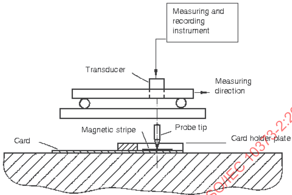
Figure 3 — Measuring device for height and profile of magnetic stripe (not to scale)
