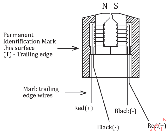
Figure 13 — Test write head coil connections (not to scale)
