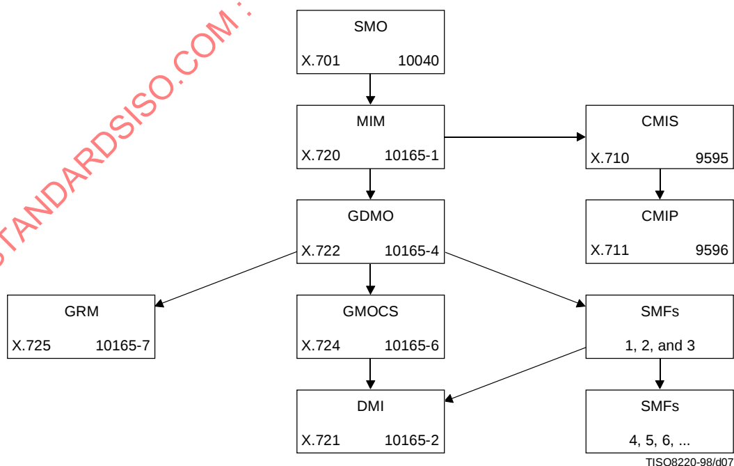
Figure 7 – Relationship between standards
