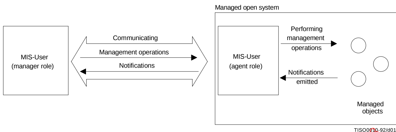
Figure 1 – Systems management interactions
