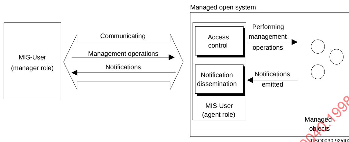
Figure 3 – Communication support for notifications and management operations
