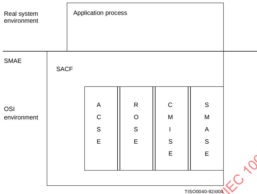
Figure 4 – Management and the application layer
