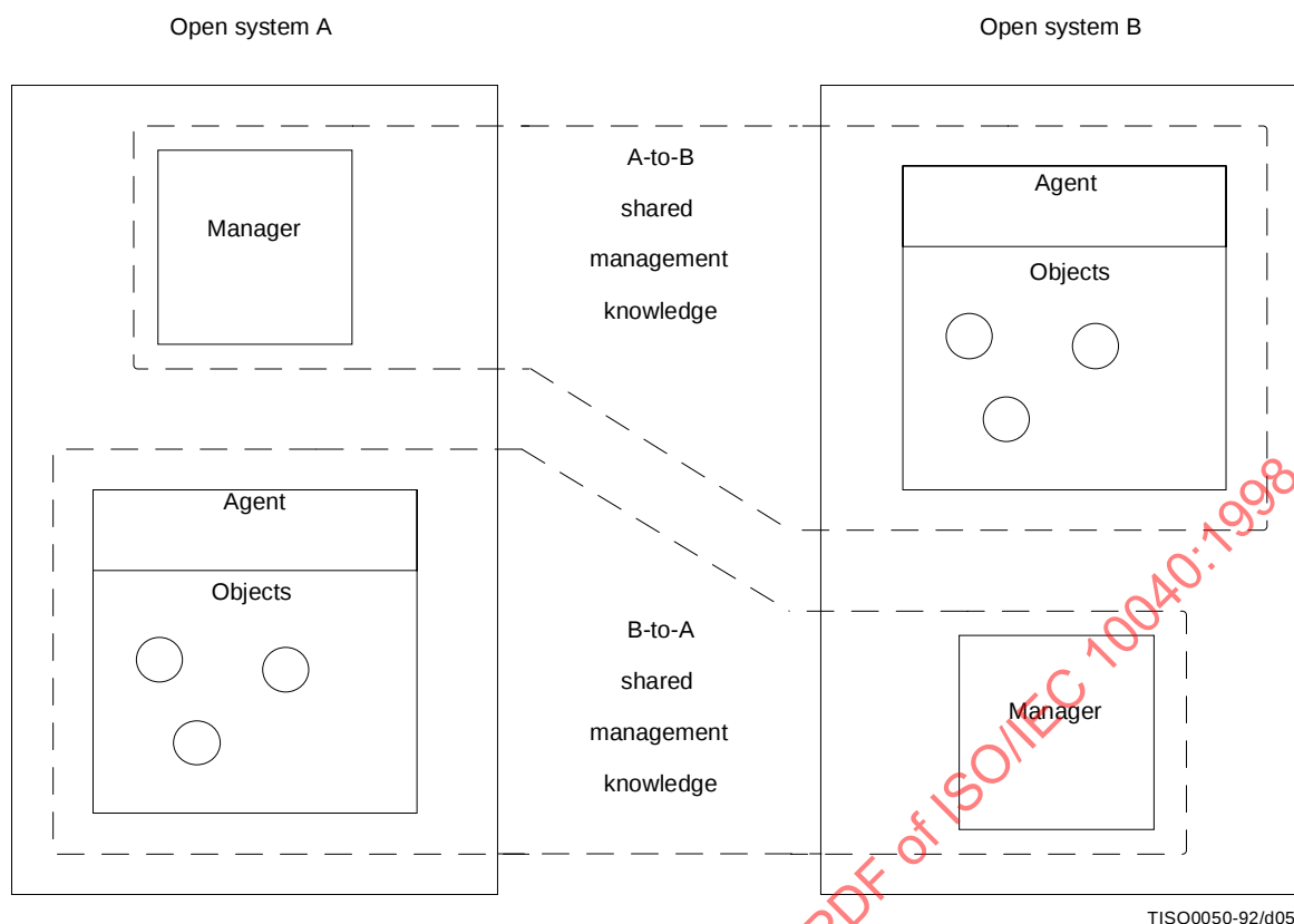
Figure 5 – Views of shared management knowledge
