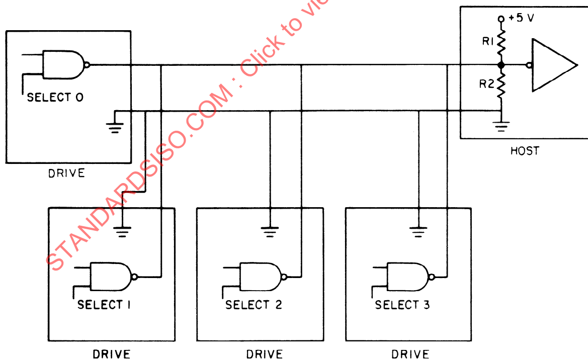
Drive-to-Host Signals
