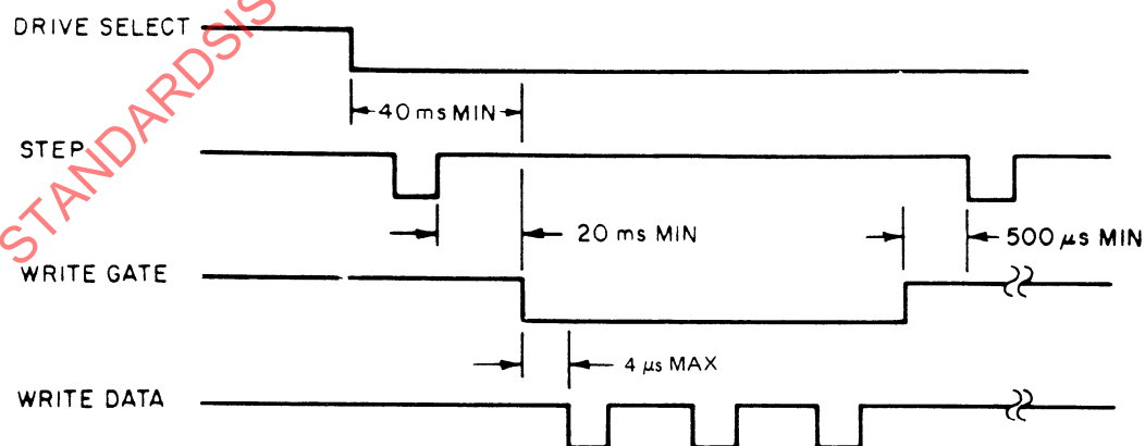
Figure 6 — Write initiate timing, 200 mm (8 in)
