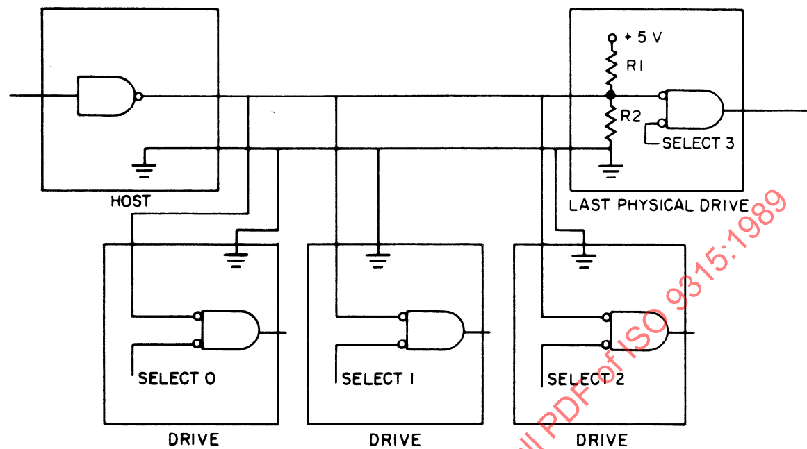
Host-to-Drive Signals
