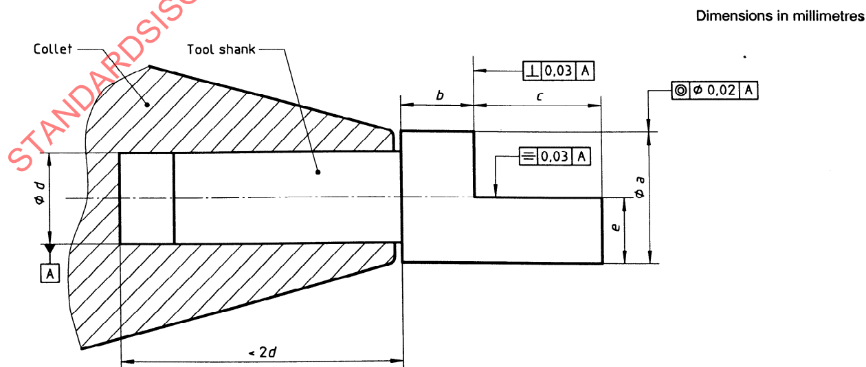
Figure 4 — Test device (inserted tool)
