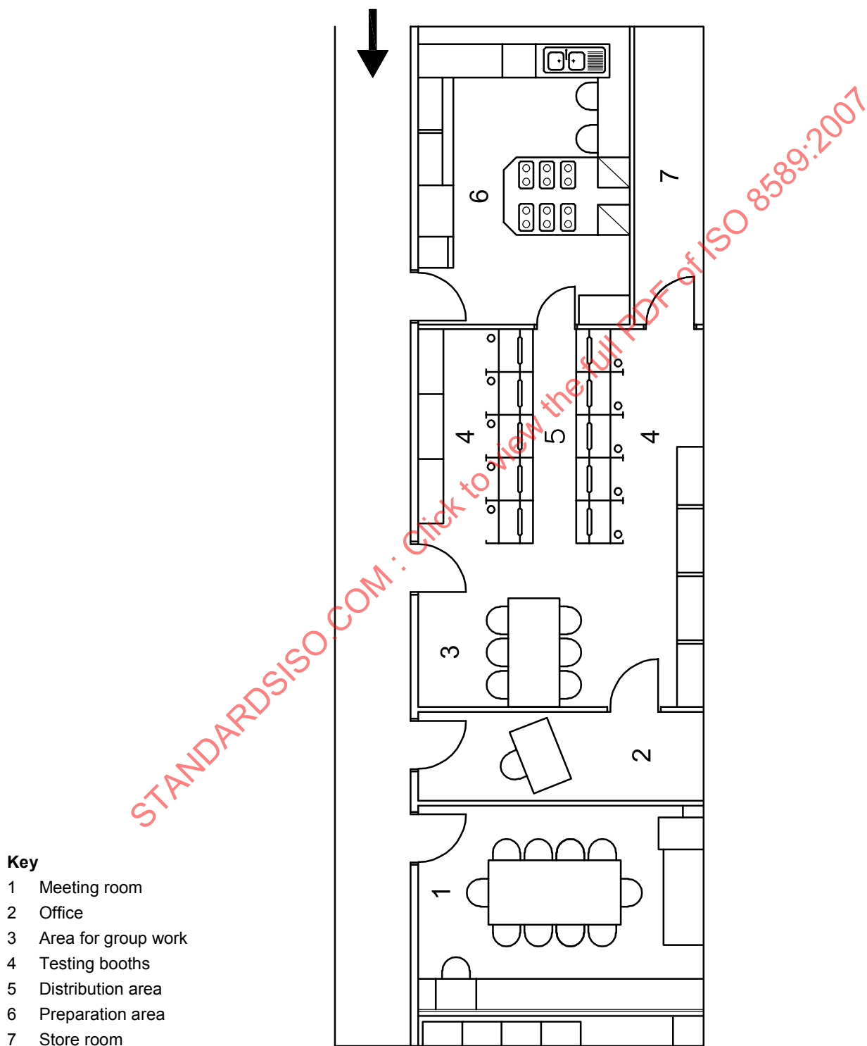
Figure A.1 — First example of a floor plan for a test room
