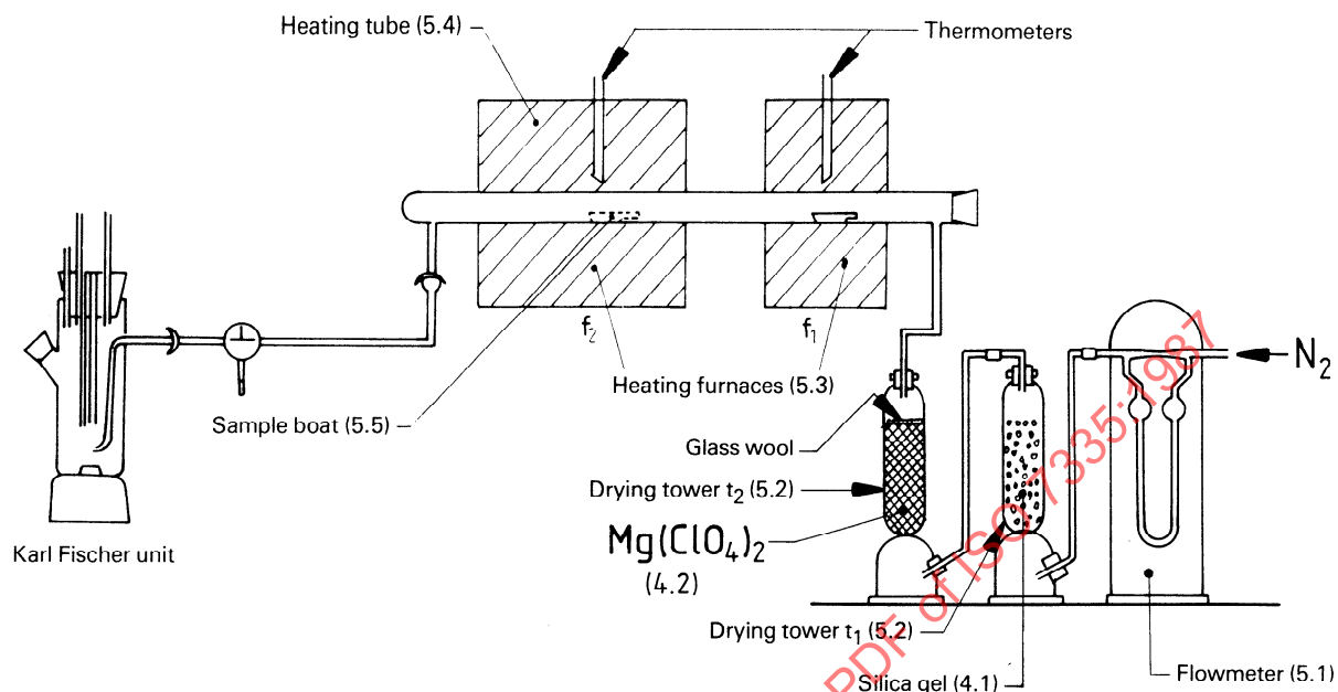
General arrangement
