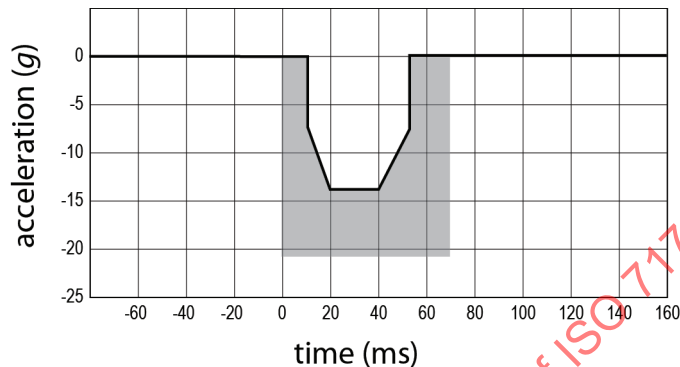
Figure G.1 — 25 km/h acceleration corridor for rear impact test
