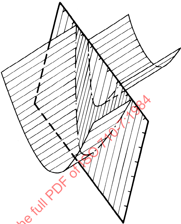
Figure 3 — Normal fault
