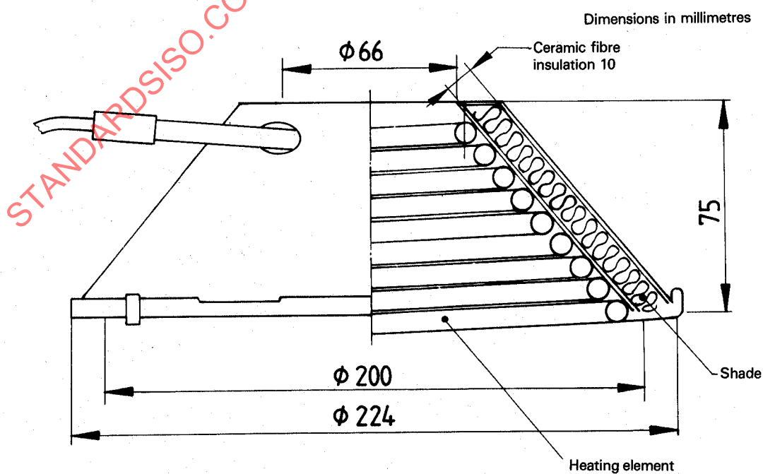
Figure 4b) — Radiator cone
