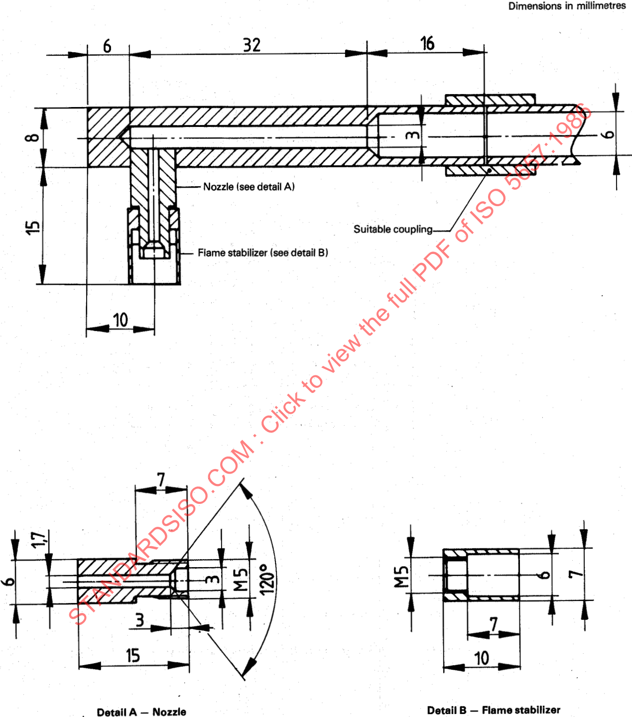
Figure 5 — Pilot flame nozzle
