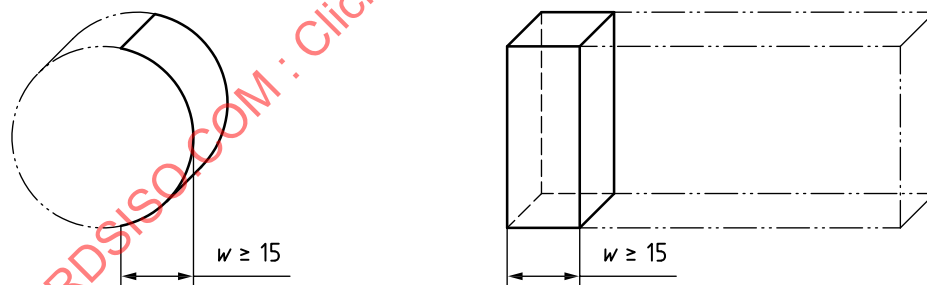
(b) Test piece taken from the sample by one cut
