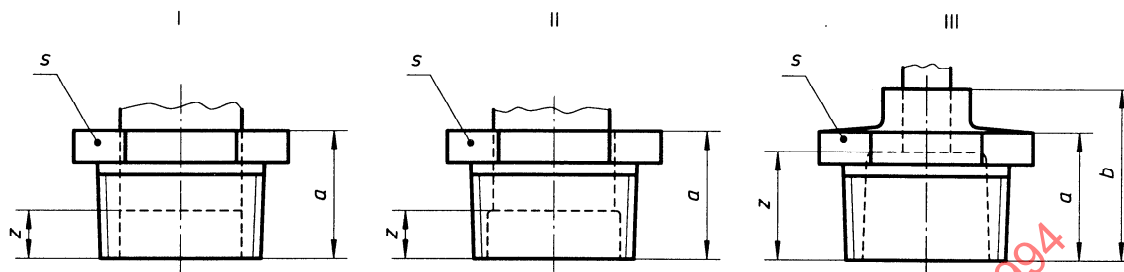
Bushings N4
