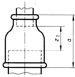
Sockets, reducing M2
