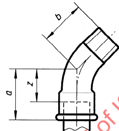
45° male and female long sweep bends G4/45°
