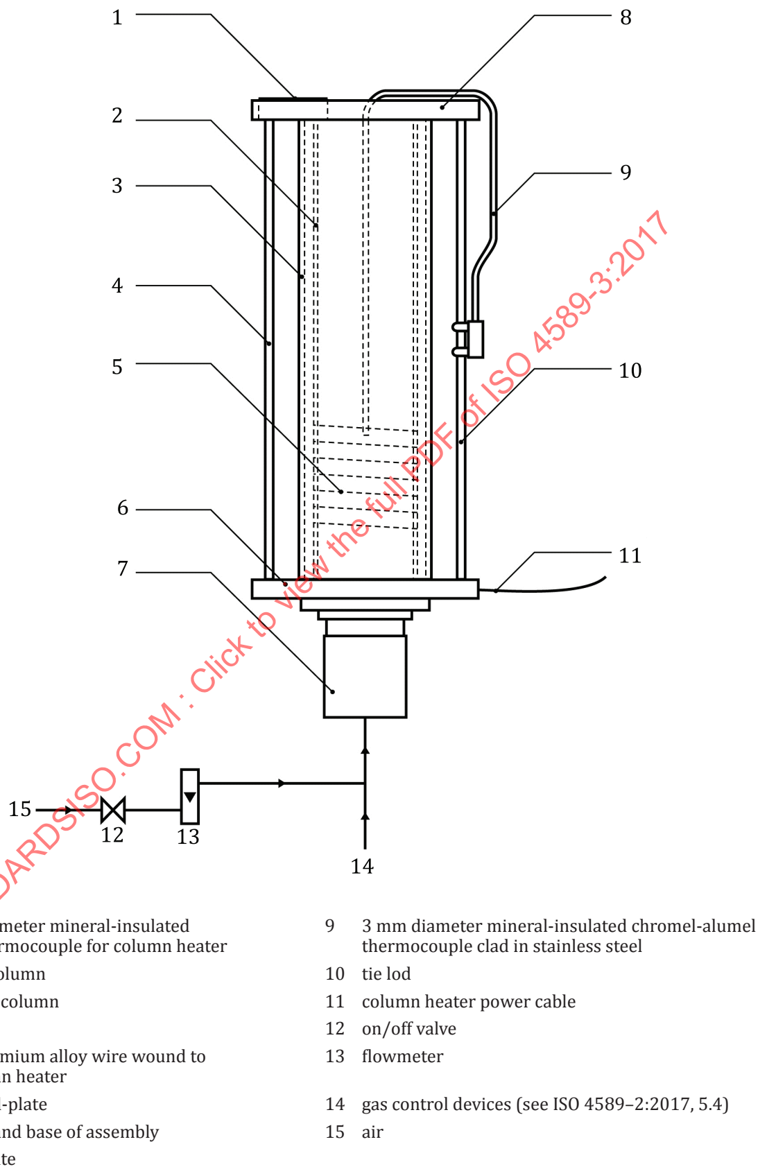
Figure 1 — Typical heated chimney
