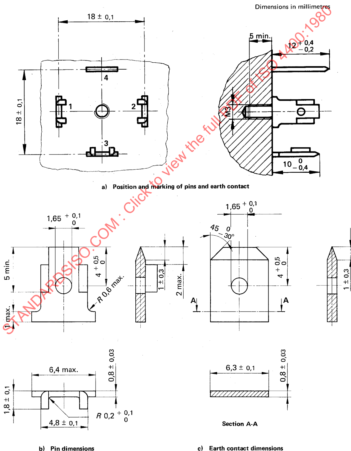
Figure 2 — Connector details
