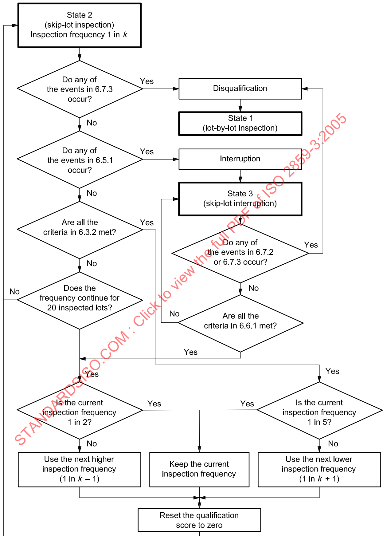
Figure 3 — Frequency shift, interruption and disqualification
