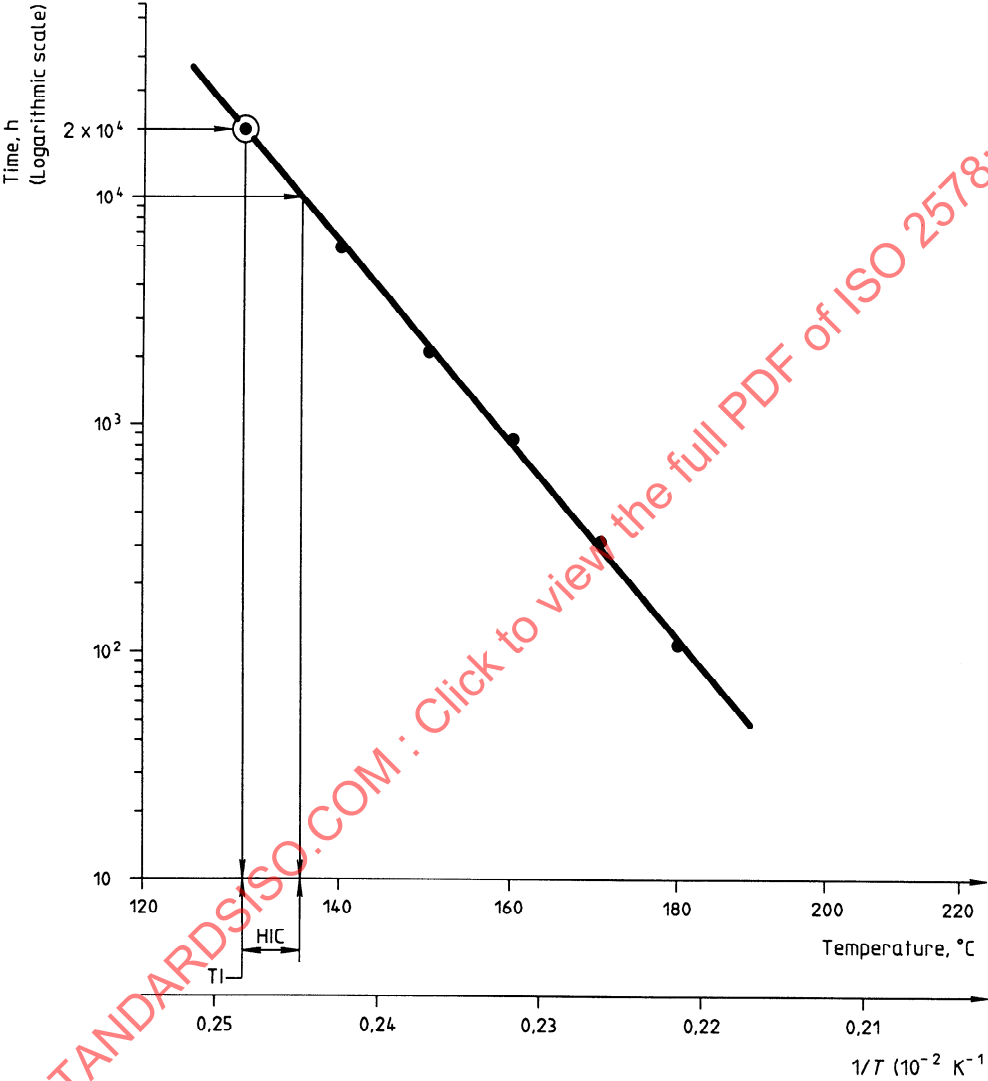
Figure 2 — Thermal endurance graph — Temperature index — Halving interval (According to IEC 216-1)
