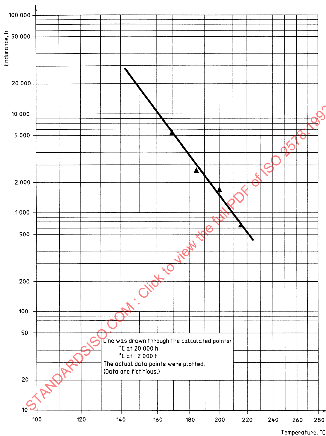
Figure A.1 — Plot of regression line based on sample calculation (see table A.2)
