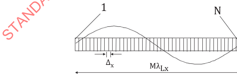
Figure B.4 — Illustration of the image sensor array along the x -direction, with element spacing \Delta_x and the measurement of the longest spatial wavelength, \lambda_{Lx} covering the total number ( N ) of pixels
