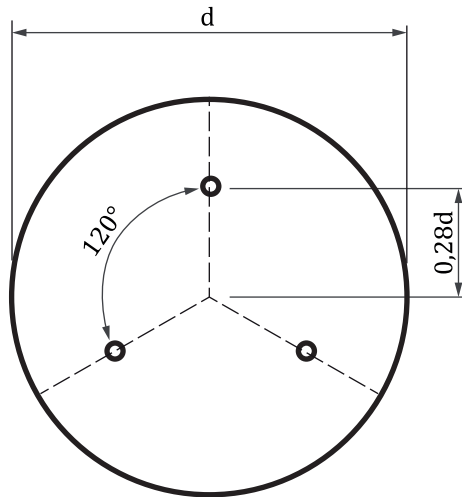
a) Position of 3 probes in a circular duct
