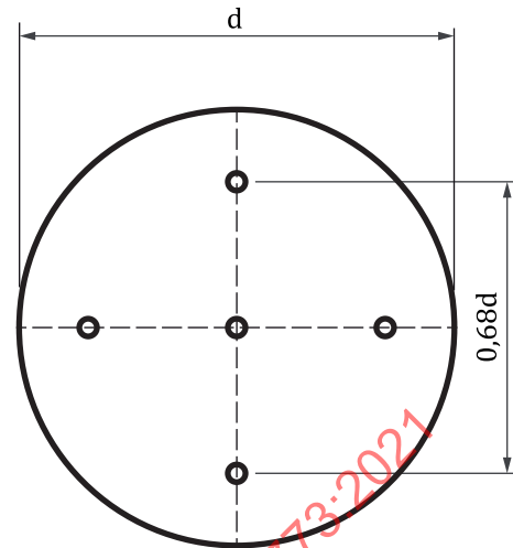
b) Position of 5 probes in a circular duct
