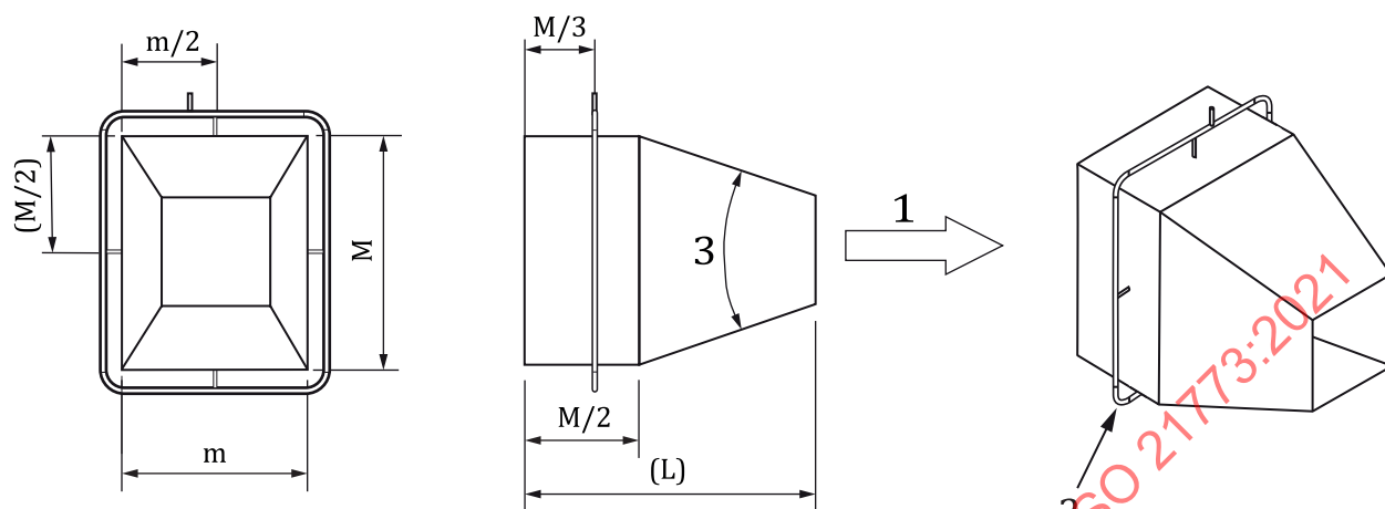
Figure B.1 — Transitions from test ducts to exchanger inlets
