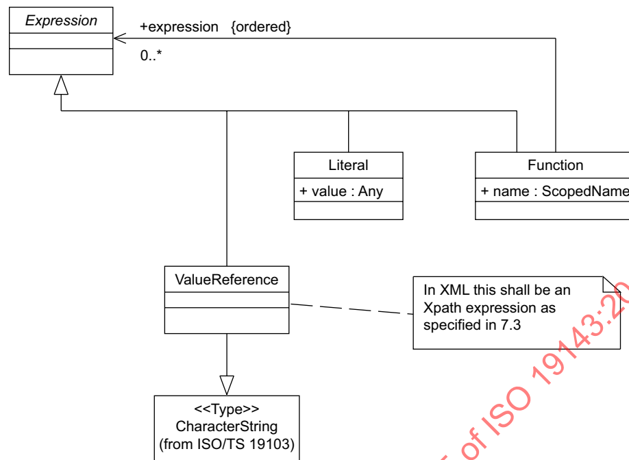
Figure 4 — Expression
