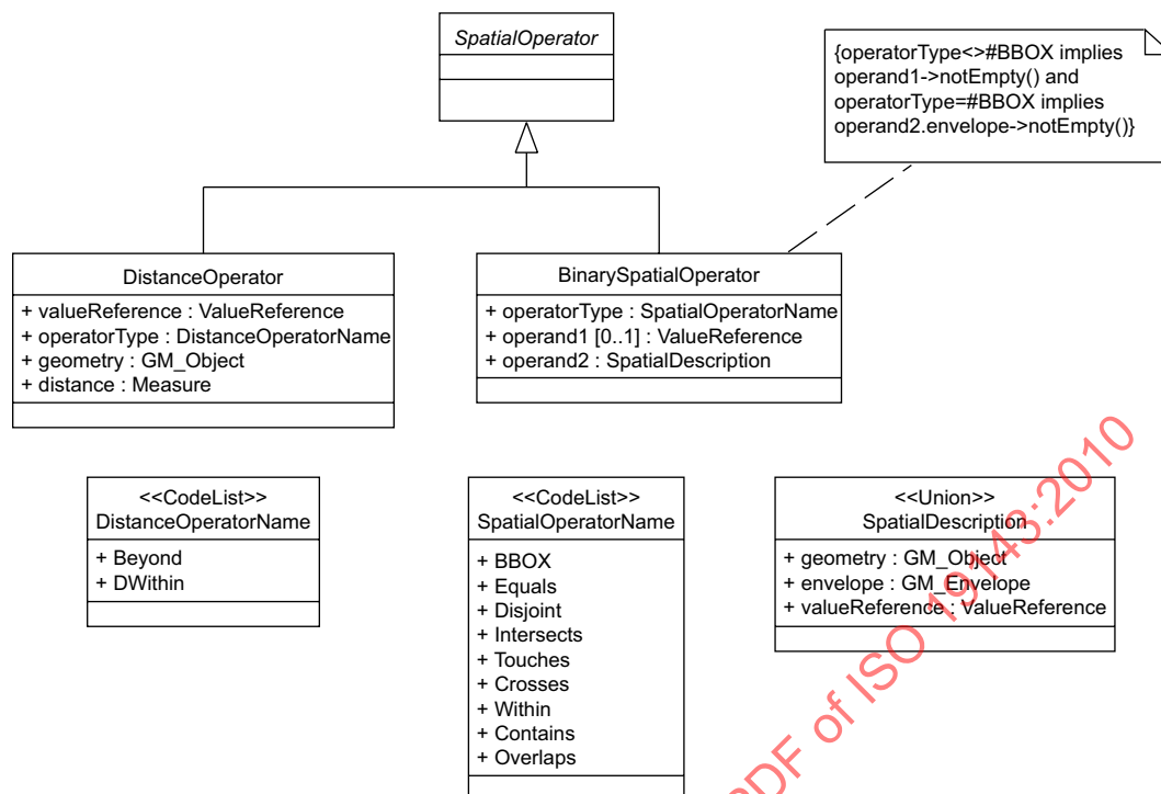
Figure 6 — SpatialOperator
