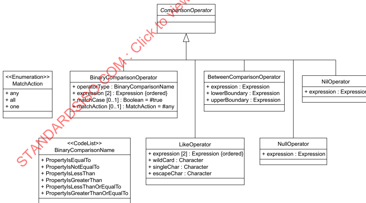
Figure 5 — ComparisonOperator
