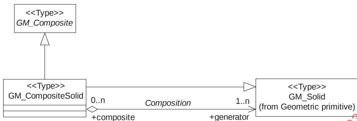
Figure 30 — GM_CompositeSolid
