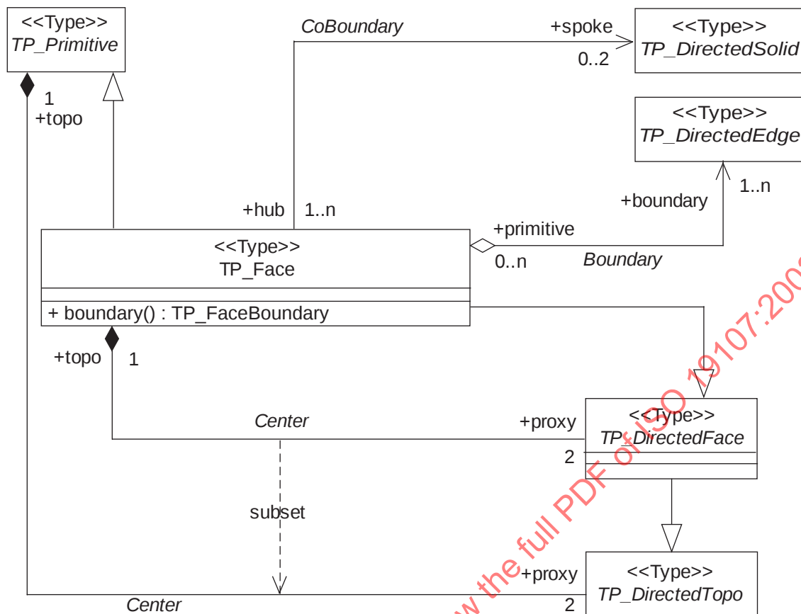
Figure 43 — TP_Face
