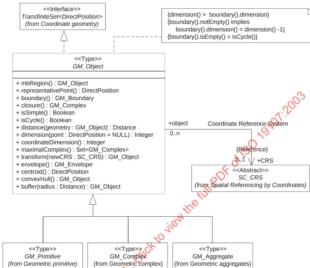
Figure 6 — GM_Object
