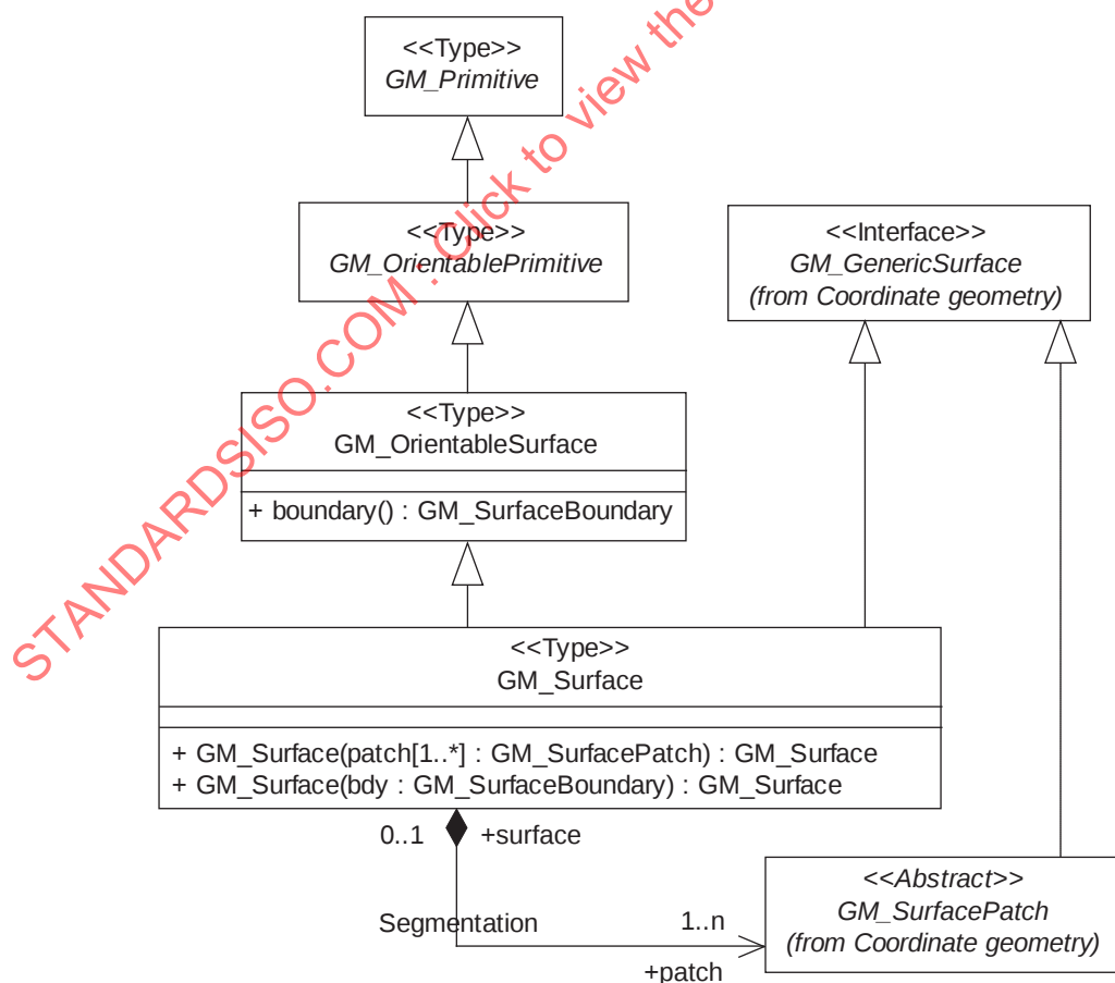
Figure 12 — GM_Surface
