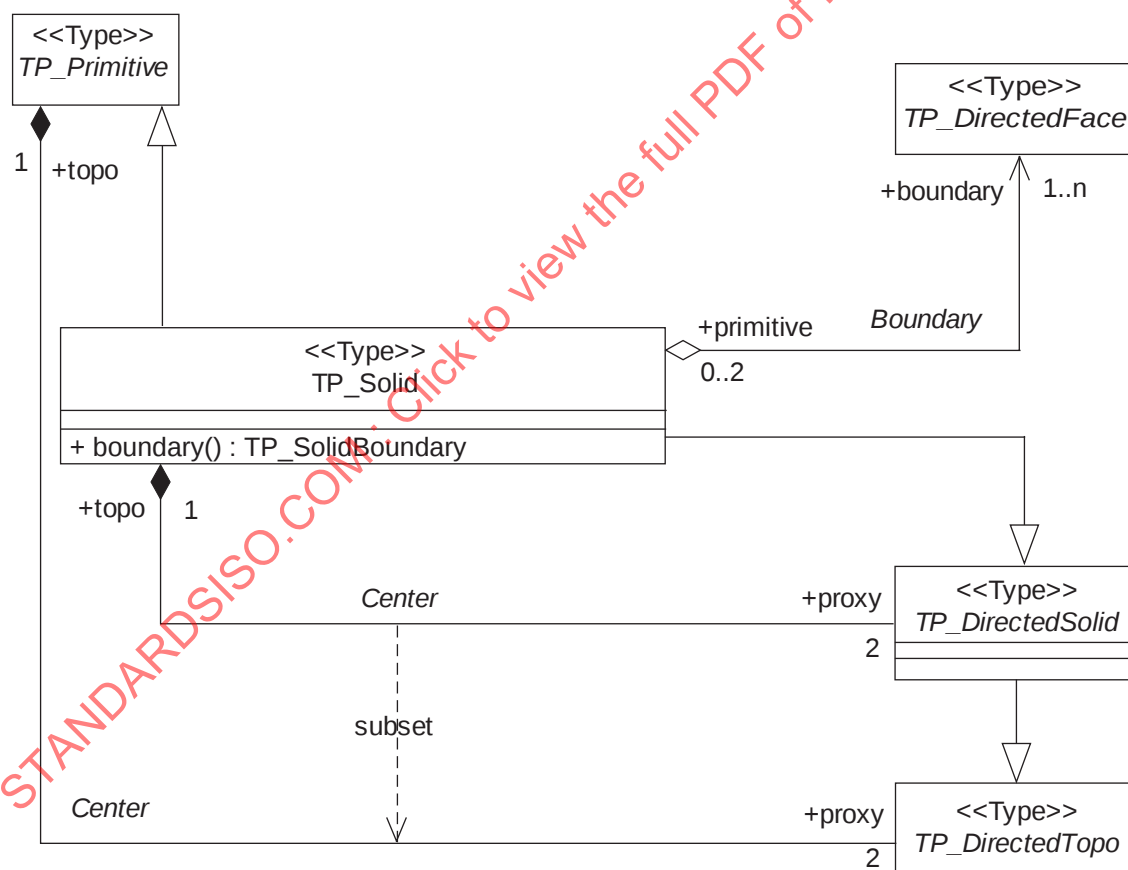
Figure 44 — TP_Solid
