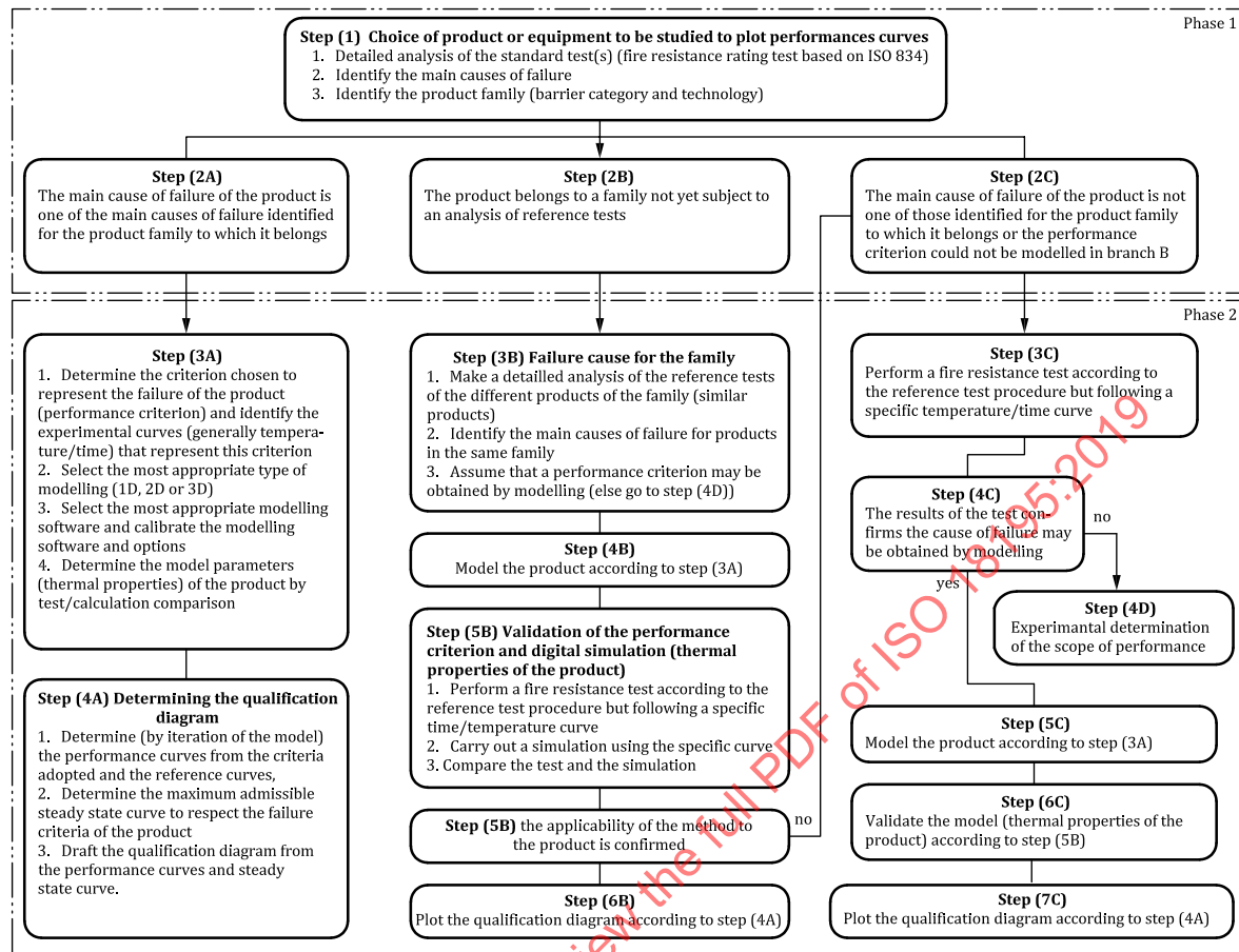
Figure 10 — Flowchart 5: Global methodology
