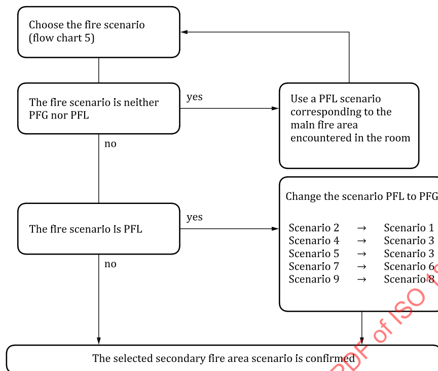
Figure 9 — Flowchart 4: selection of a secondary source scenario
