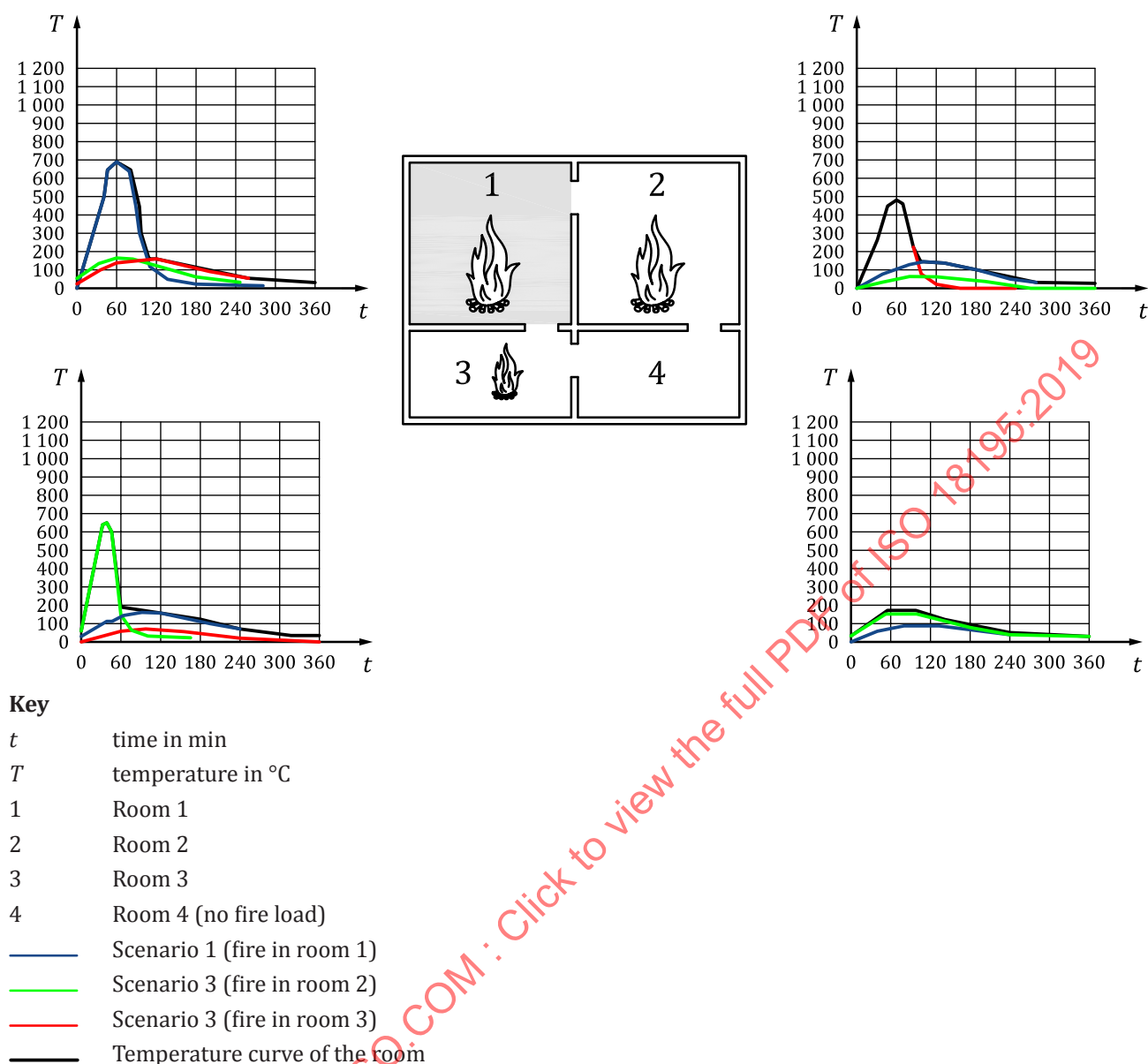
Figure 5 — Design basis fire temperature curve construction
