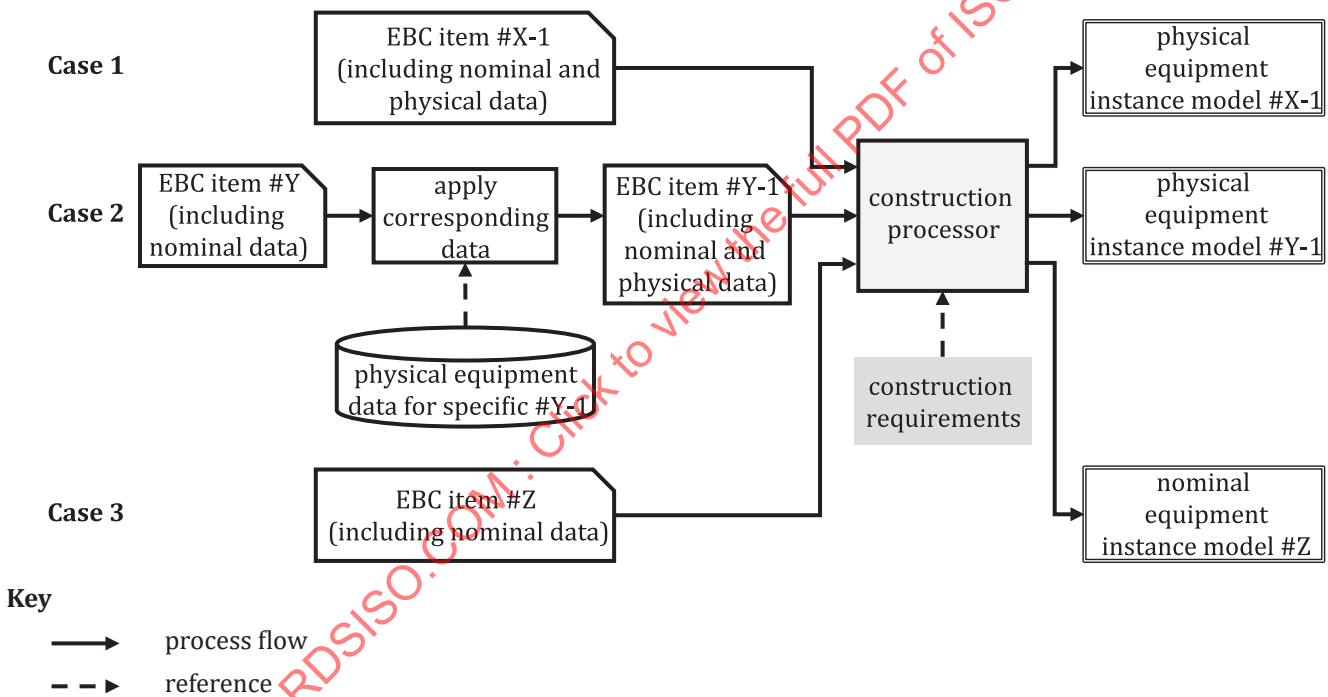
Figure 2 — Construction of an equipment instance model
