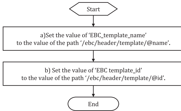
Figure B.2 — Step A using Rule 1
