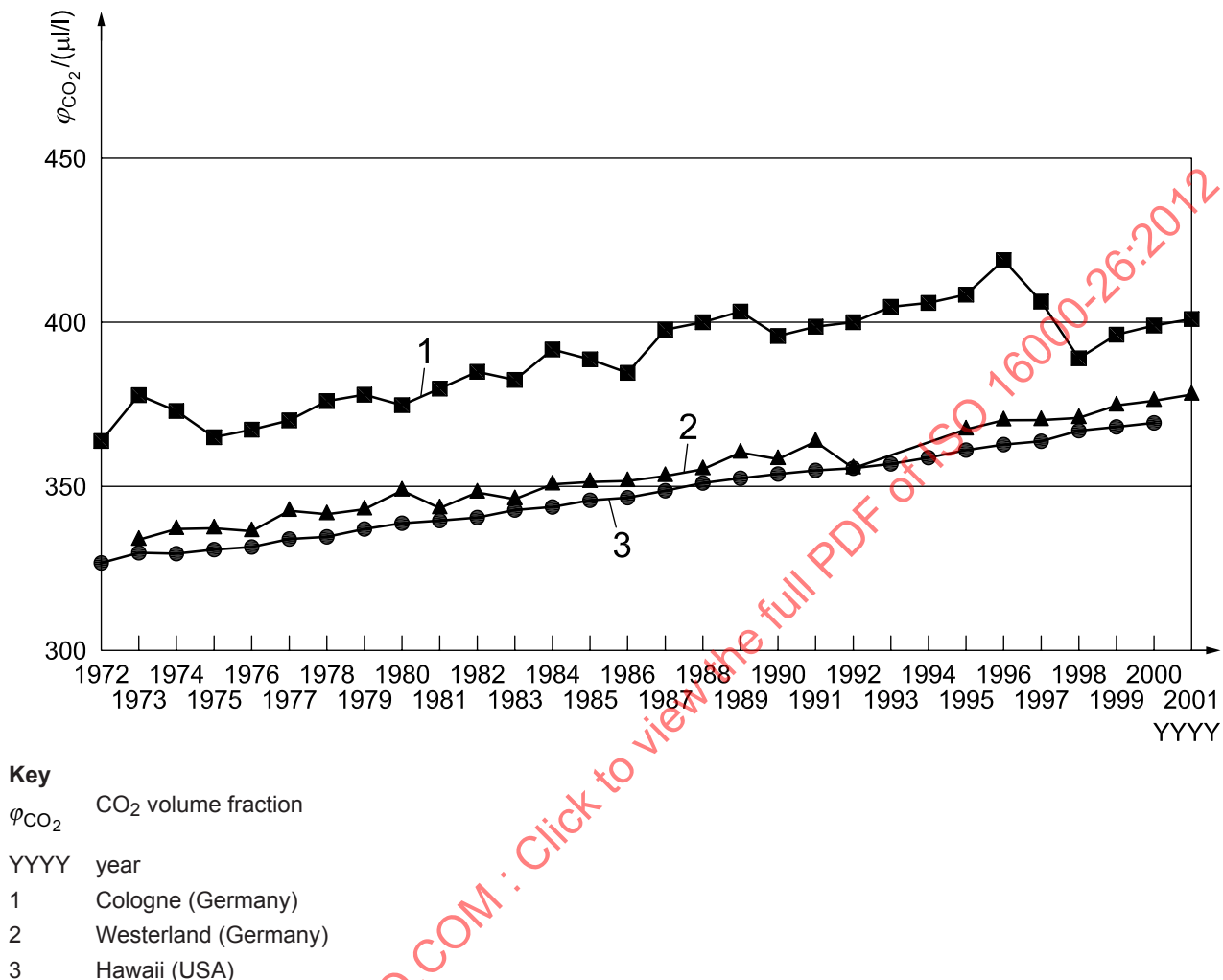
Figure 1 — Annual mean values of the CO 2 concentrations in ambient air at various locations
