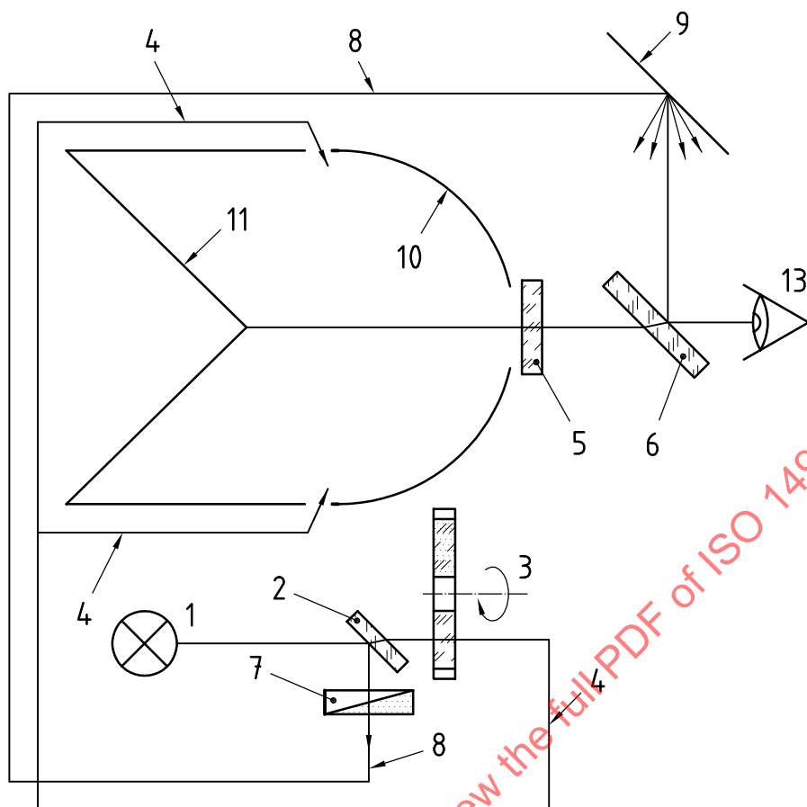
a) Operation in transmission
