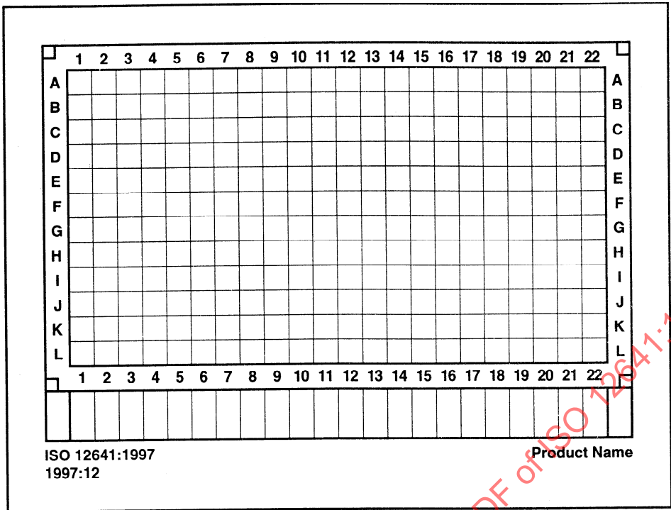
Figure 6 — Layout, colour reflection target
