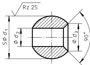
Figure 3 — Type Z3, ball-type nozzle
