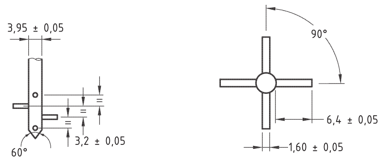
Figure 2 — Stirrer rabble arms
