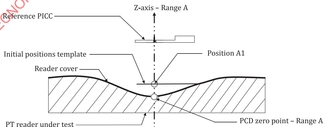
Figure 10 — Testing a symmetric concave-surface PT reader
