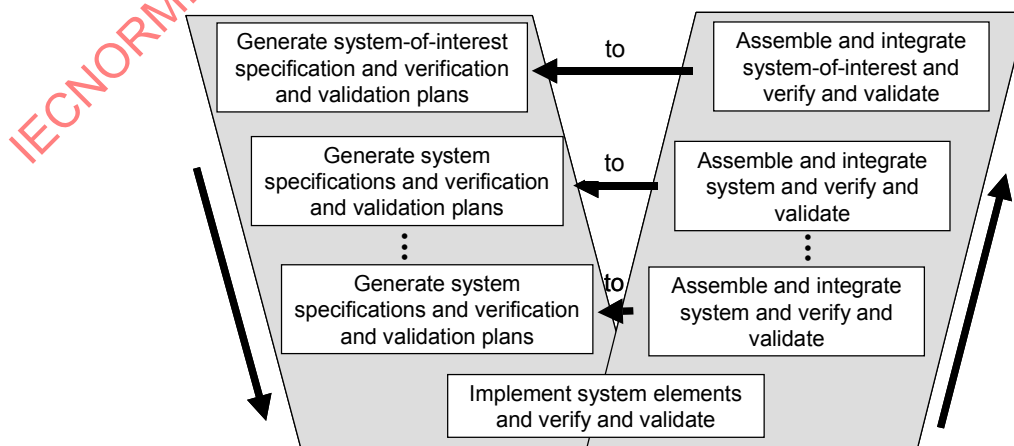
Figure 23 — The engineering "Vee" model
