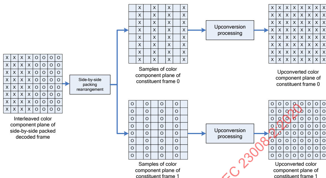
Figure D.5 — Rearrangement and upconversion of side-by-side packing arrangement with frame_packing_arrangement_type equal to 3, quincunx_sampling_flag equal to 0, ( x , y ) equal to ( 12, 8 ) for constituent frame 0, and ( x , y ) equal to ( 0, 0 ) or ( 4, 8 ) for constituent frame 1
