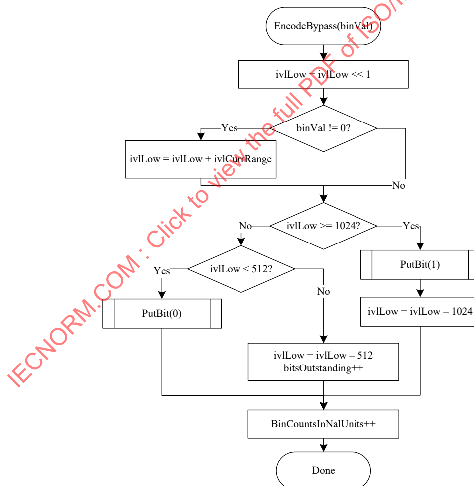
Figure 9-13 — Flowchart of encoding bypass
