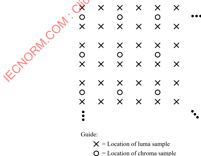
Figure 6-1 — Nominal vertical and horizontal locations of 4:2:0 luma and chroma samples in a picture
