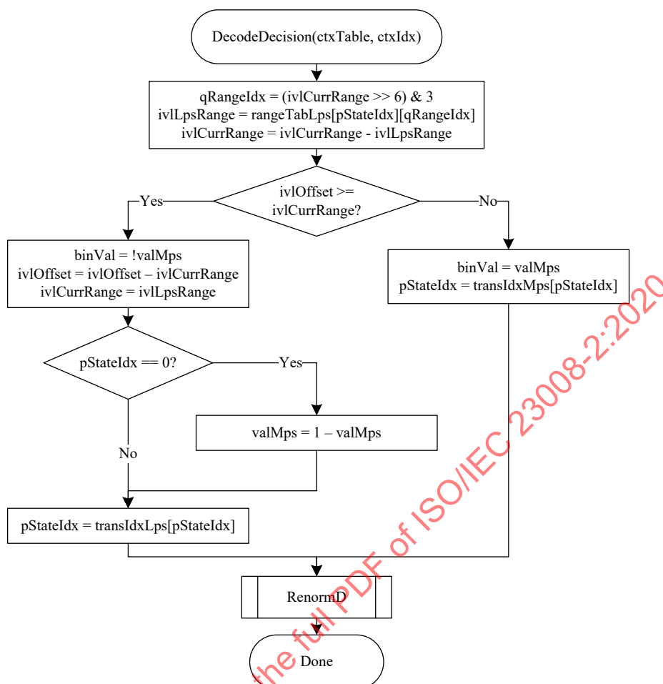
Figure 9-6 — Flowchart for decoding a decision
