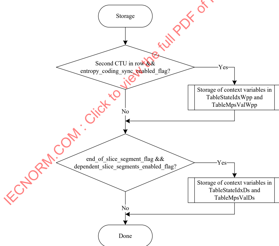
Figure 9-4 — Illustration of CABAC storage process
