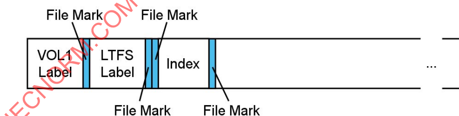
Figure 4 — Partition Layout
