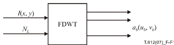
Figure F.1 – Inputs and outputs of the FDWT procedure
