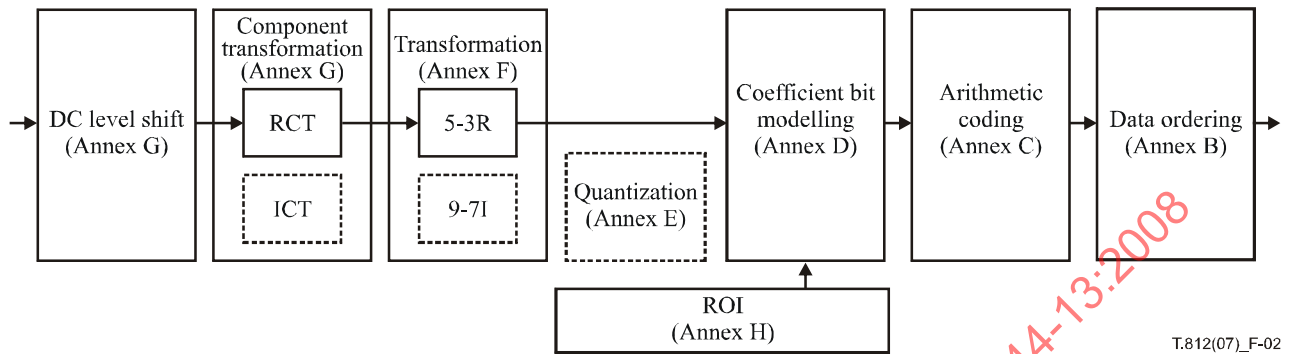
Figure 2 – Lossless based colour encoding block diagram
