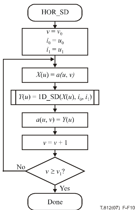
Figure F.10 – The HOR_SD procedure
