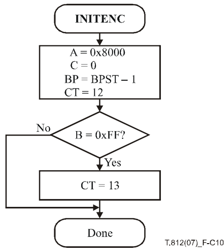
Figure C.10 – Initialization of the encoder
