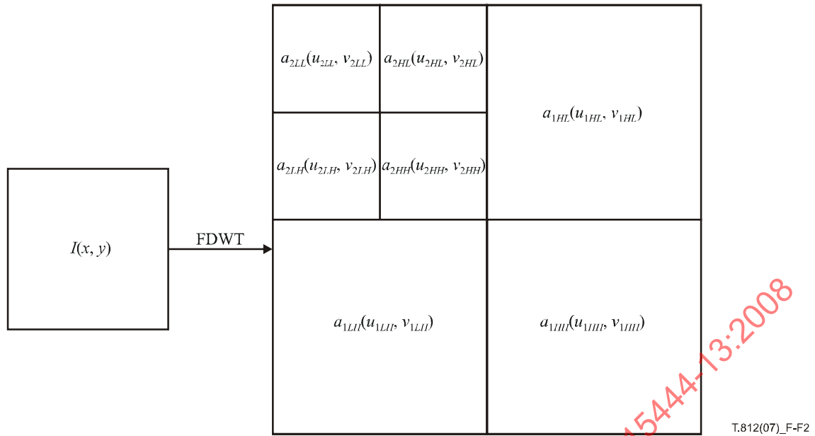
Figure F.2 – The FDWT ( N_L = 2 )
