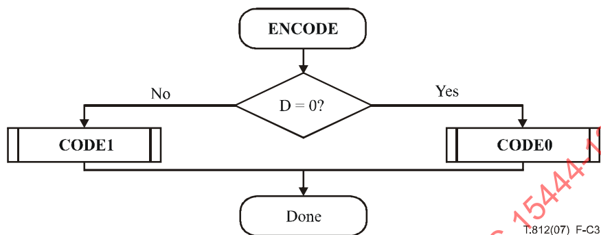
Figure C.3 – ENCODE procedure
