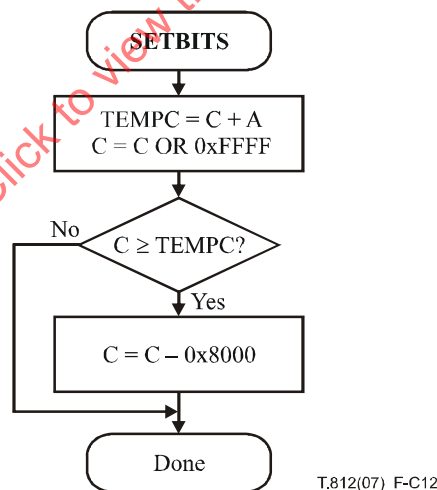
Figure C.12 – Setting the final bits in the C register
