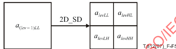
Figure F.5 – One-level decomposition into four sub-bands (2D_SD procedure)
