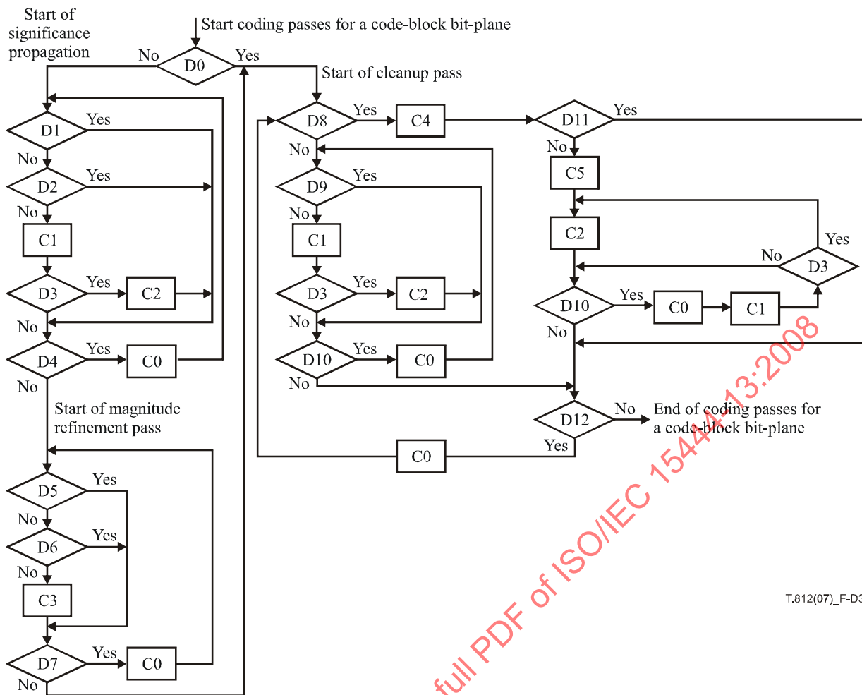
Figure D.3 – Flow chart for all coding passes on a code-block bit-plane
