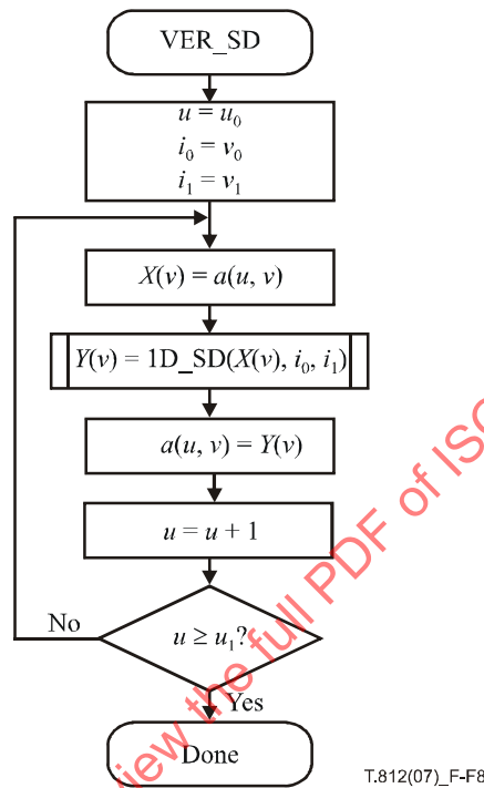
Figure F.8 – The VER_SD procedure
