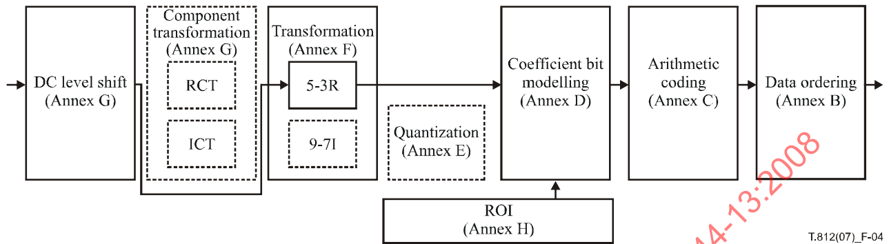
Figure 4 – Lossless based greyscale encoding block diagram
