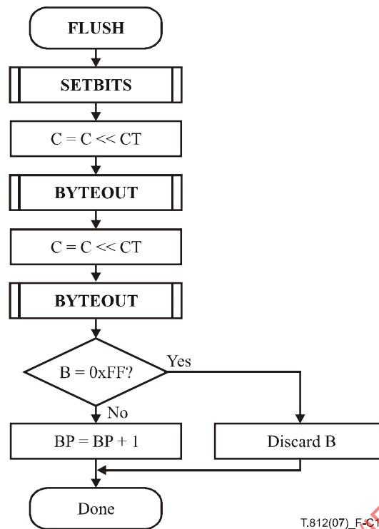
Figure C.11 – FLUSH procedure
