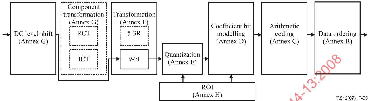
Figure 5 – Lossy based greyscale encoding block diagram
