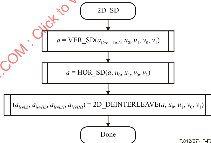
Figure F.6 – The 2D_SD procedure
