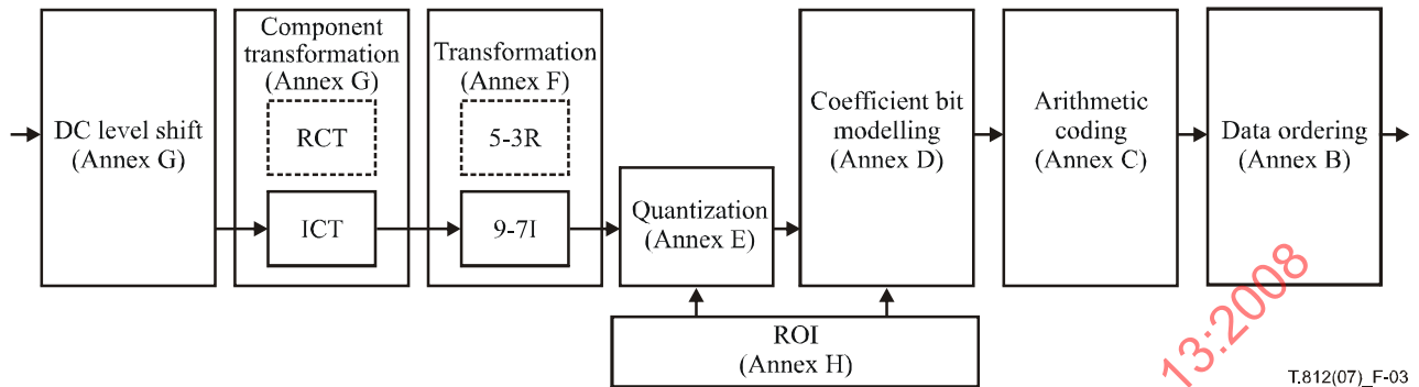
Figure 3 – Lossy based colour encoding block diagram
