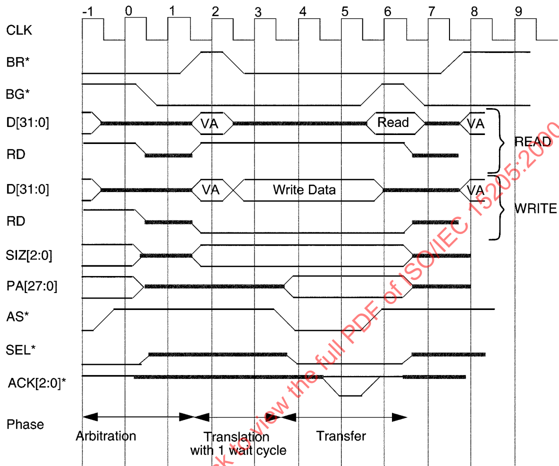
Figure 13 – Example of 32-bit symmetric SBus cycle
