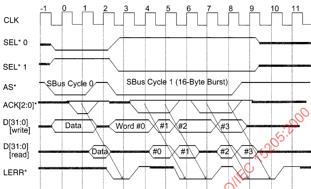
Figure 11 – Example of LERR* timing
