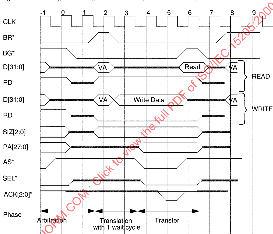
Figure 14 – Example of 64-bit Extended Transfer symmetric SBus cycle
