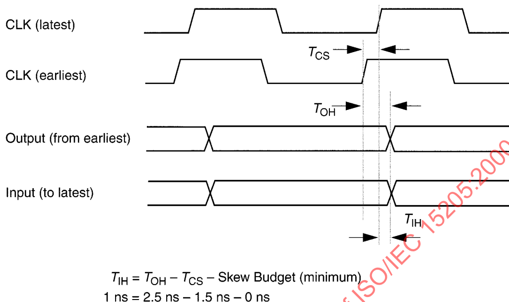
Figure 22 – Output and input hold time relationships, including clock skew
