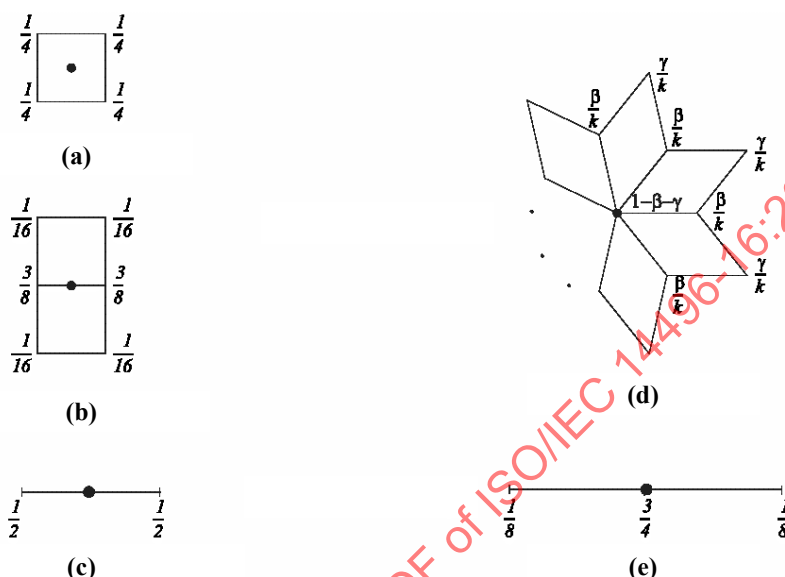
Figure 12 — Catmull-Clark rules with k defined as in subclause 3.3.2.1.2 (a) face rule; (b) regular edge rule (c) boundary/crease edge rule (d) interior vertex rule \beta = 3/2k and \delta = 1/4k (e) smooth boundary/crease vertex rule
