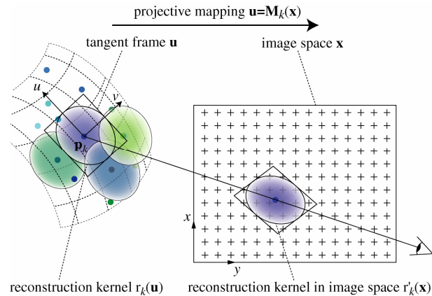
Figure 28 — Local tangent planes and reconstruction kernels
