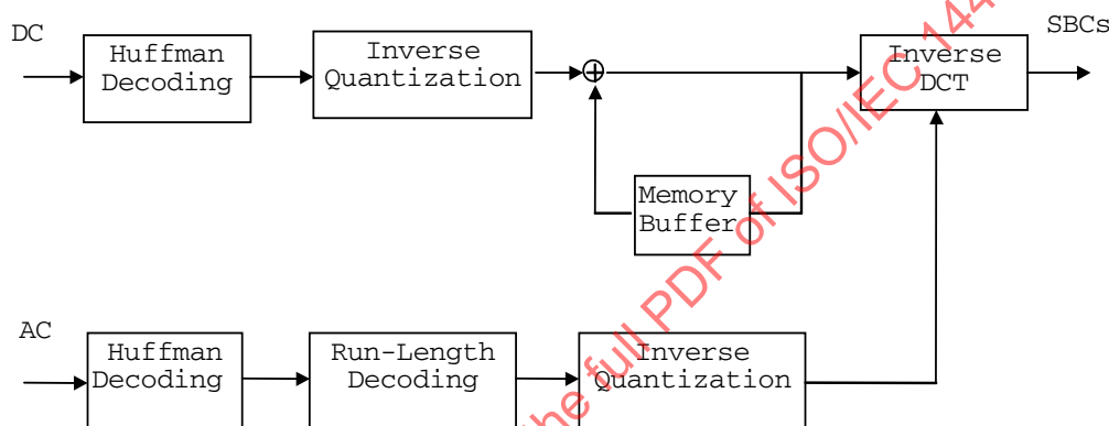
Figure 74 — Block diagram of the DCT-based SBCs decoding process.
