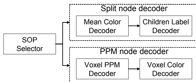
Figure 69 — Block diagram of tree node decoder.
