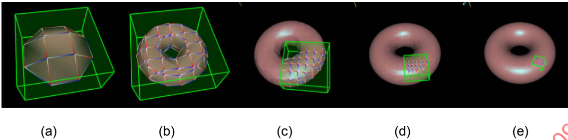
Figure 45 — Different resolution levels of a multi-resolution MeshGrid can be coded as one mesh (view-independent coding) or split into several ROI (view-dependent coding).
