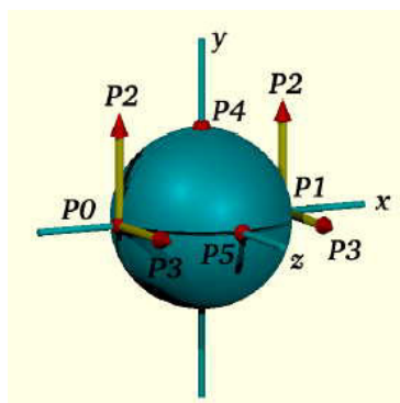
Figure 24 — Quadric's 6 geometric control points
