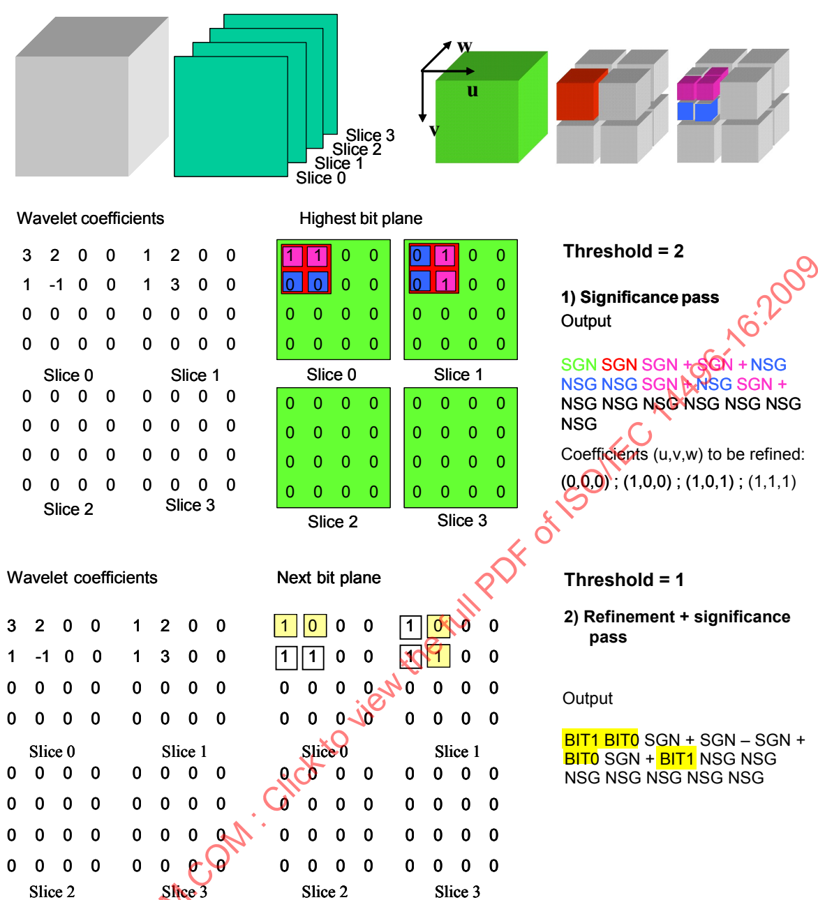
Figure 58 — Graphical representation of the significance and refinement coding passes.
