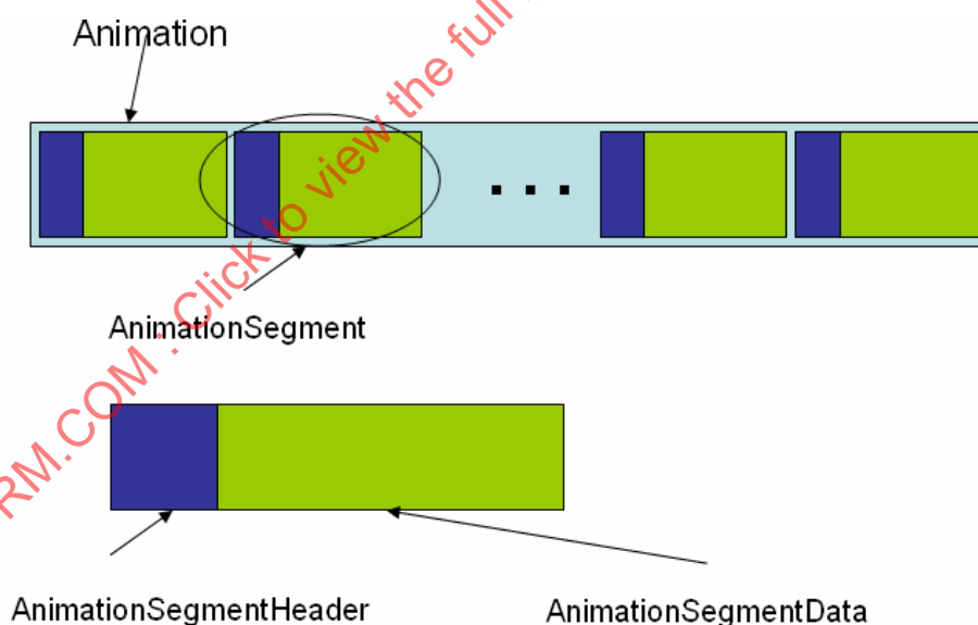
Figure 75 — FAMC bitstream structure.
