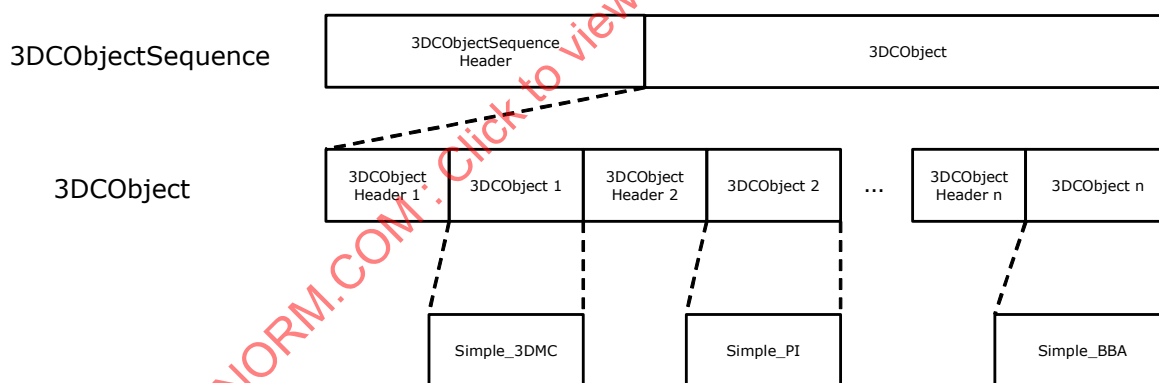
Figure 77 — Syntax of the MP43D stream
