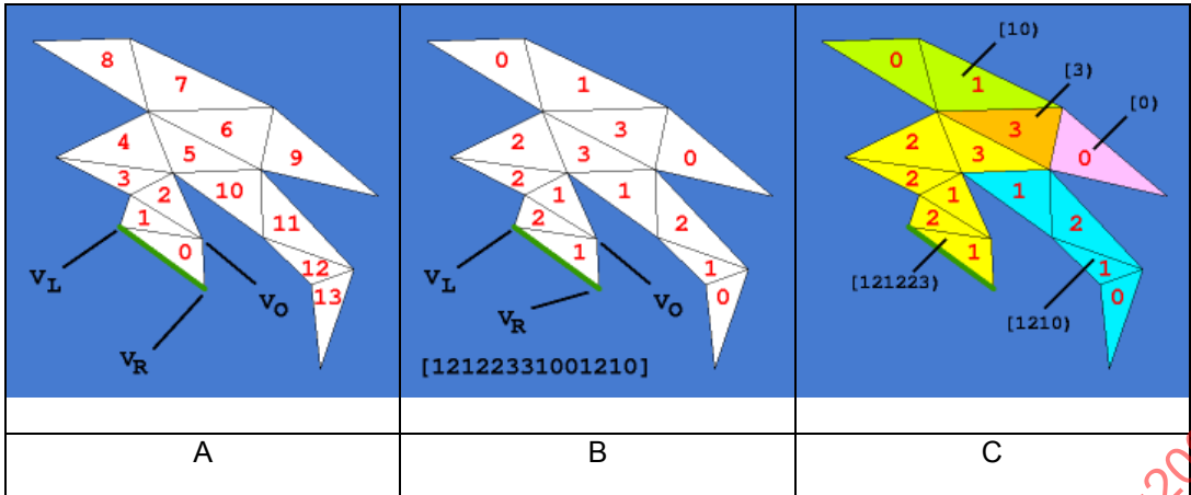
Figure 38 — Representing a simple polygon as a table of triangle runs.
