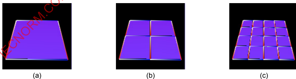
Figure 61 — Example of a multi-resolution mesh with the connectivity-wireframe obtained by uniformly splitting each quad recursively into four sub-quads.
