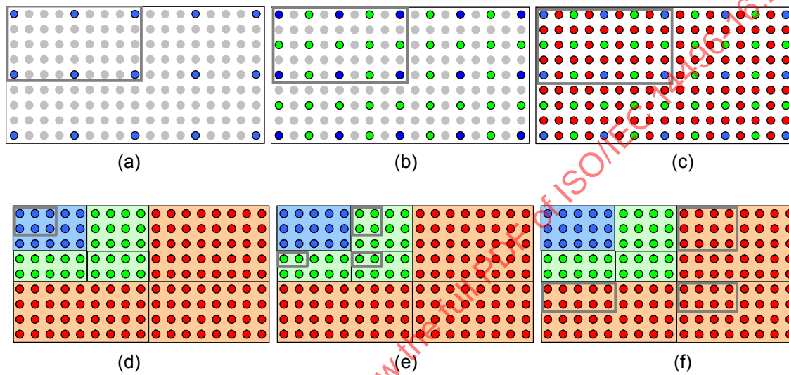
Figure 60 — A slice through the 3D reference-grid illustrating: (1) the distribution of the grid-points in the spatial domain (a, b, c) (resolution I, I+1, I+2) and in the wavelet domain (d, e, f), (2) the correspondence between a ROI defined at different resolutions in the spatial domain and its corresponding WROIs in the wavelet domain.
