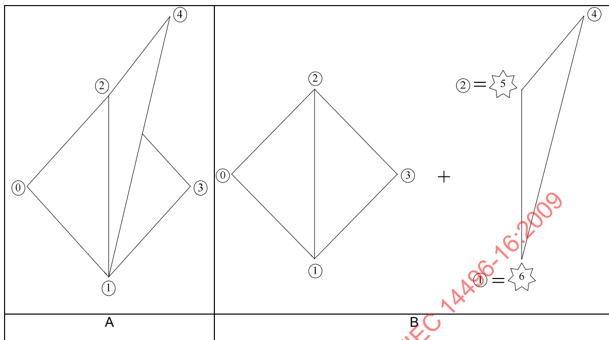
Figure 39 — A non-manifold 3D mesh (A) and converted manifold meshes (B)
