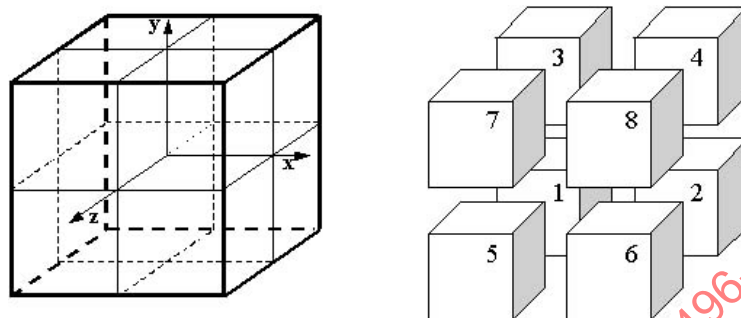
Figure 27 — The structure of octree and the order of the children
