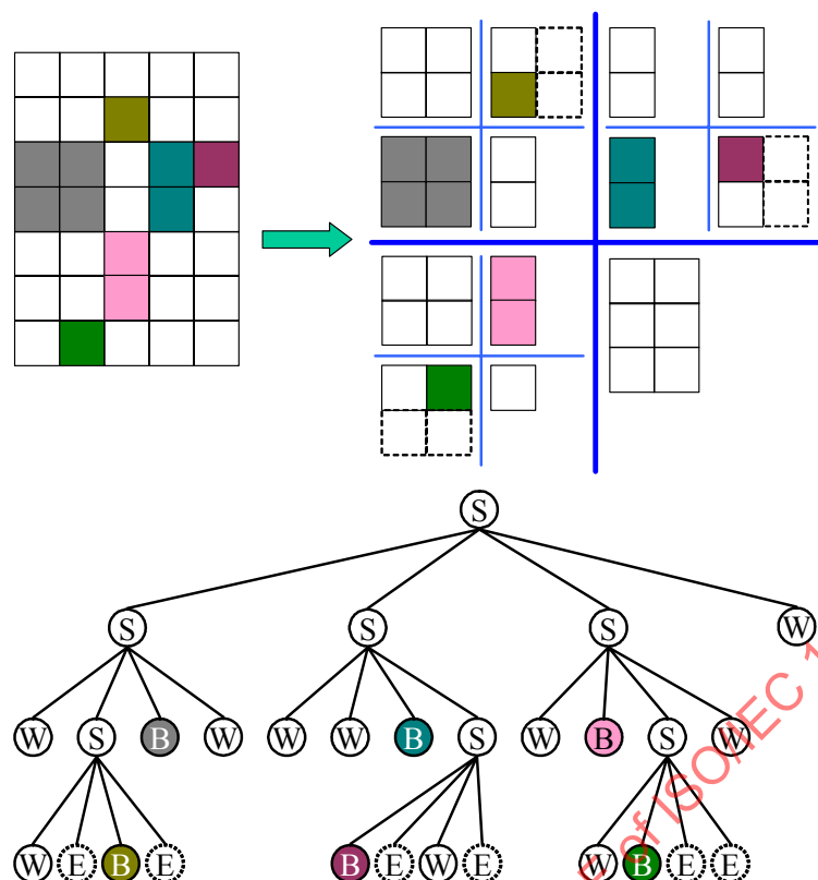
Figure 65 — Example of adjustable octree in the resolution of 5x7.
