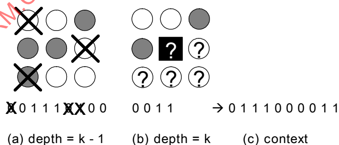
Figure 70 — Example of context: a voxel represented by a question marked black square in (b) is the voxel to be decoded and voxels represented by white circles and gray circles in (a) and (b) are used to make a context excluding three voxels which are marked with 'X'.
