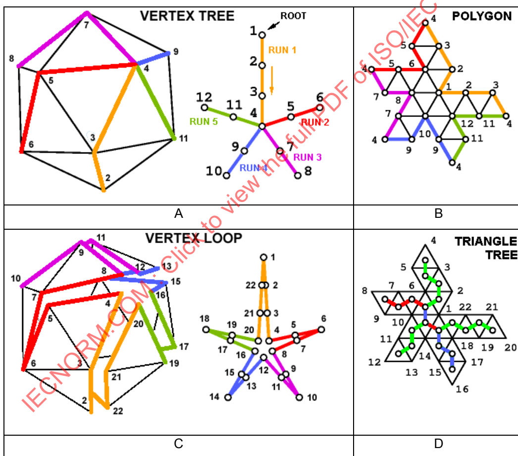
Figure 35 — Topological Surgery representation of a simple mesh.
