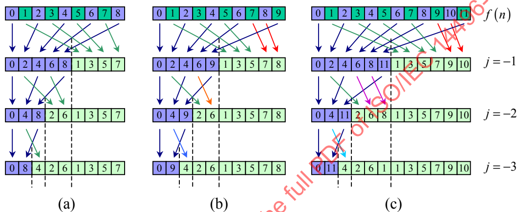
Figure 57 — Graphical illustration of the wavelet decomposition for odd and even-length signals.
