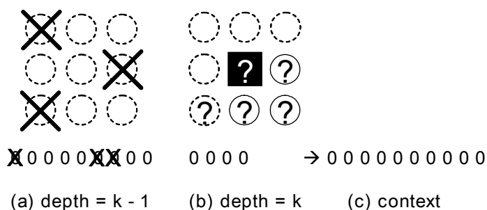
Figure 71 — Example of context: voxels represented by dotted circles in (a) and (b) are not existed voxels and a voxel to be decoded in (b) is located at a corner actually.
