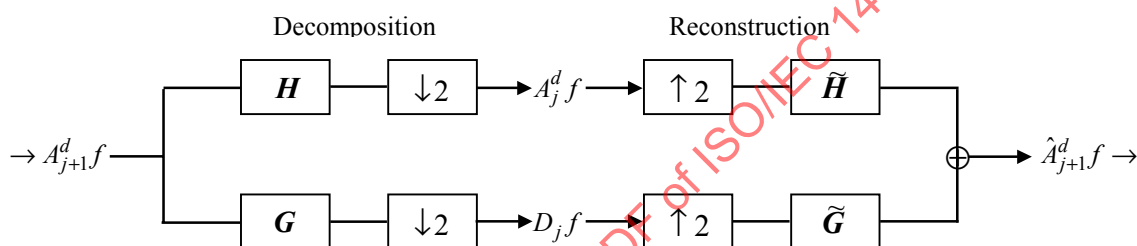
Figure 56 — Wavelet decomposition and reconstruction of a 1D signal.
