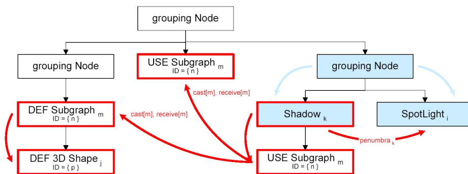
Figure 30 — Transmission of shadow properties to 3D-surfaces and light sources
