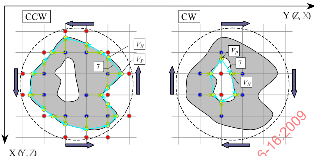
Figure 48 — A cross-section through a 3D object, illustrating the scanning direction, which is CCW for an external surface and CW for an internal surface. The connectivity vectors have the orientation of the scanning direction.
