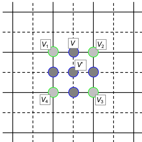
Figure 62 — Computation of the offsets for the type2 quadrilateral MeshGrid.
