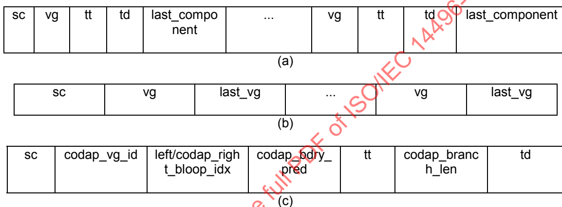
Figure 36 — Types of data partition: (a) one or more group of vg, tt and td included in a partition. (b) one or more vgs included in a partition. (c) the partition has one pair of tt and td.
