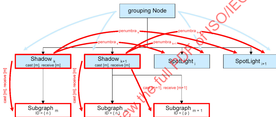
Figure 31 — Transmission of shadow properties to multiple 3D-surfaces and light sources
