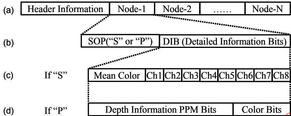
Figure 66 — Example of the bitstream structure for compressed PointTexture.
