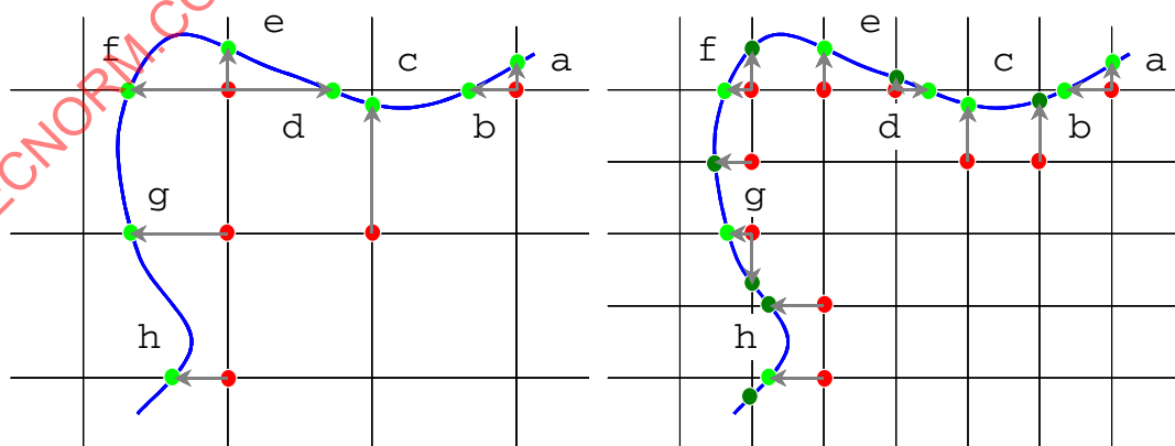
Figure 59 — Demonstration of vertex migration via the Inter-Resolution Refinement bits. The labelled vertices from the lower resolution Mesh-Description (left image) will migrate (some of them) to new reference-grid positions in the next higher resolution level (right image). For the sequence of vertices abcdefgh, the refinement bits are: 00110110, which means that vertices a, b, e, and h will not migrate while the others do.
