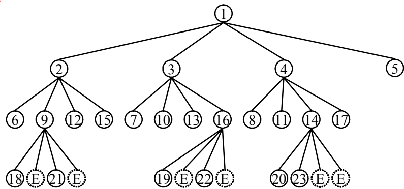
Figure 68 — Example of the decoding order for the tree nodes in Figure 66.
