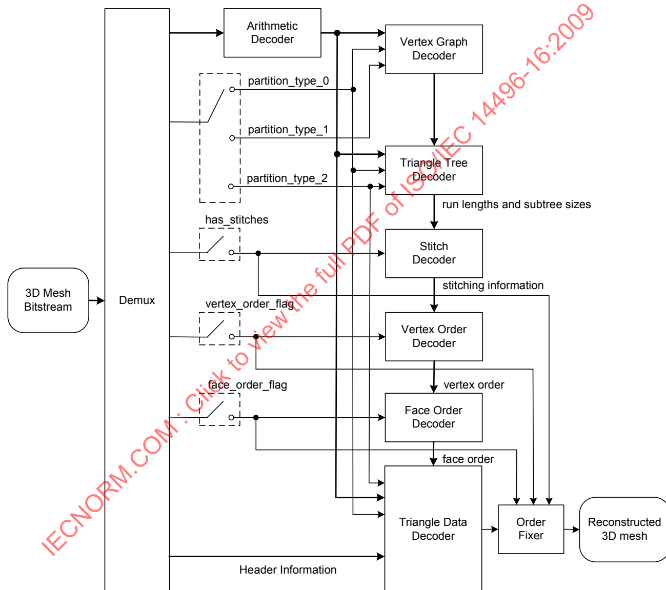
Figure 34 — Block diagram of the Topological Surgery decoder
