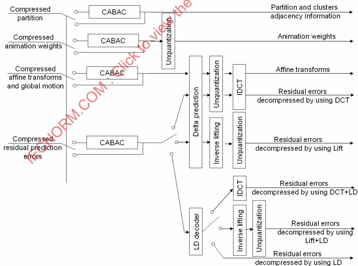
Figure 76 — FAMC decoding process.
