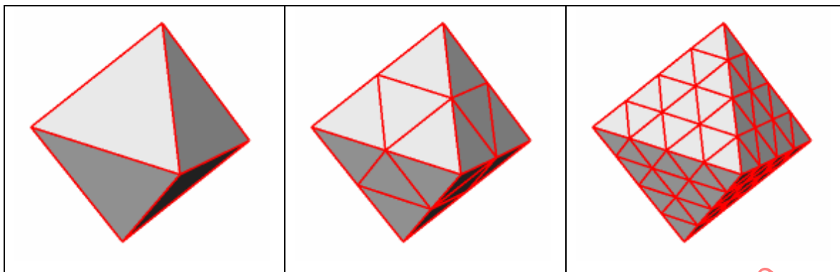
Figure 43 — The quantisation of normals is based on the hierarchical subdivision of the unit octahedron.
