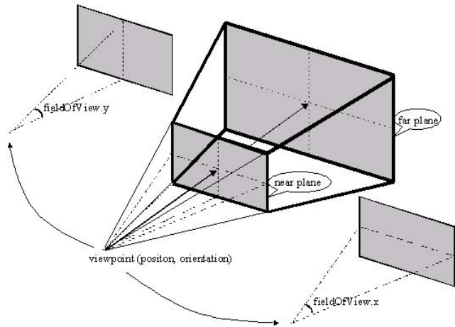
Figure 25 — Perspective view of the DepthImage
