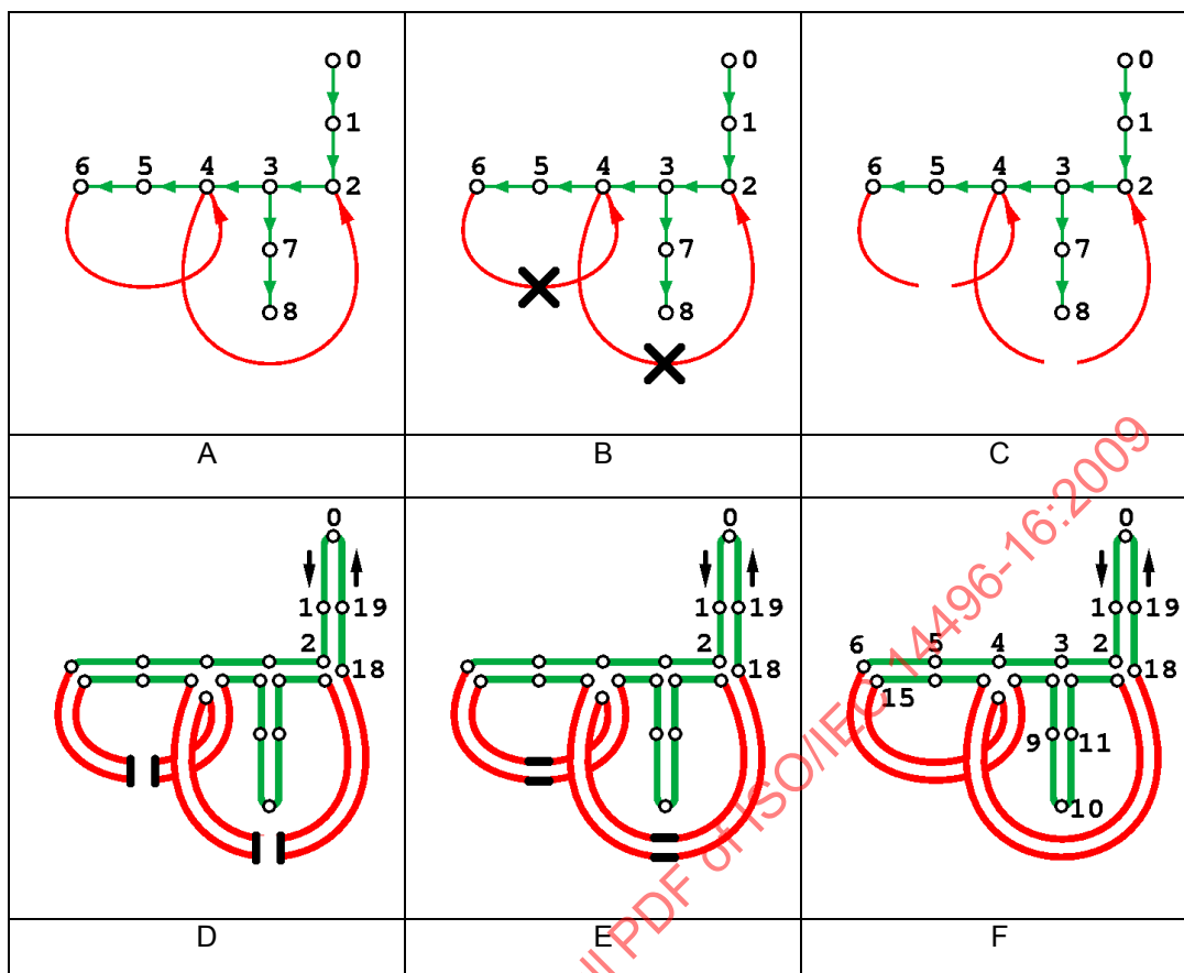
Figure 37 — Steps to build the bounding loop from the vertex graph. A: vertex graph decomposed into vertex tree (green) and jump edges (red). B: extended vertex tree is created by cutting jump edges in half. C: the extended vertex tree has two leaves for each jump edge. D: build the extended vertex tree loop. E: connect the start and end of each jump edge. F: resulting boundary loop.
