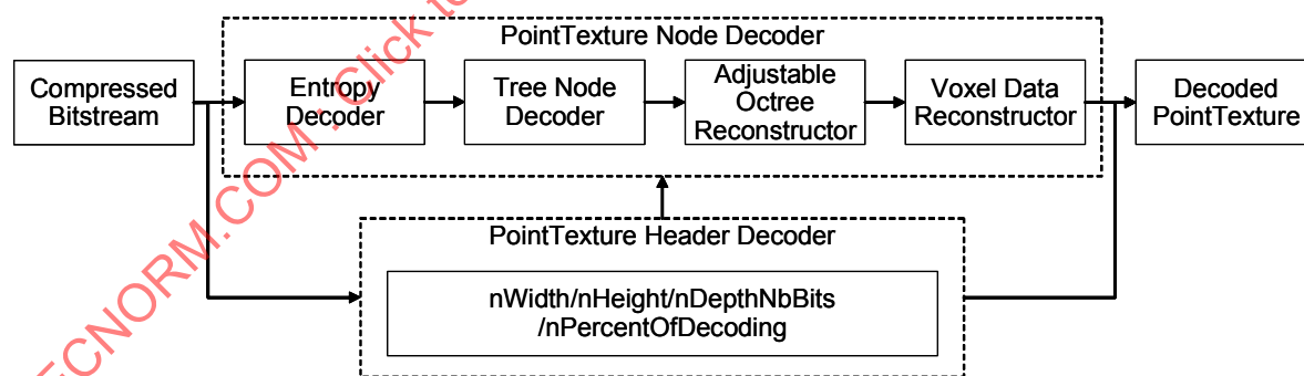
Figure 63 — Block diagram of decoder for PointTexture compression.
