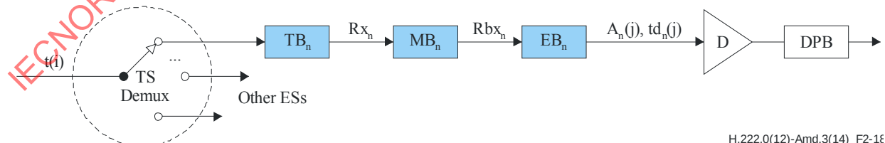
Figure 2-18 – T-STD model extensions for single layer HEVC
