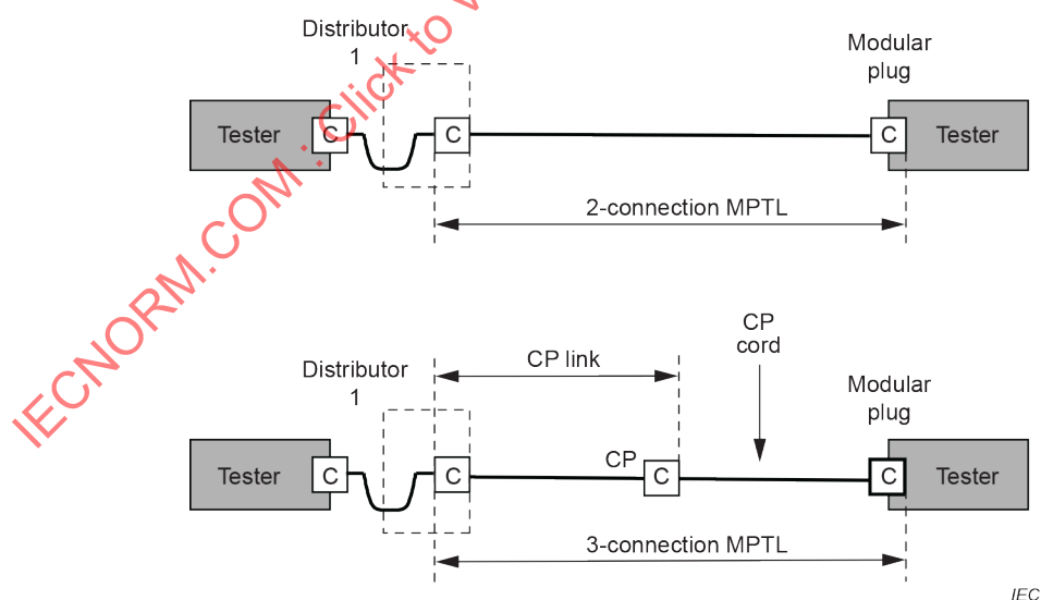
Figure 1 – MPTL configurations
