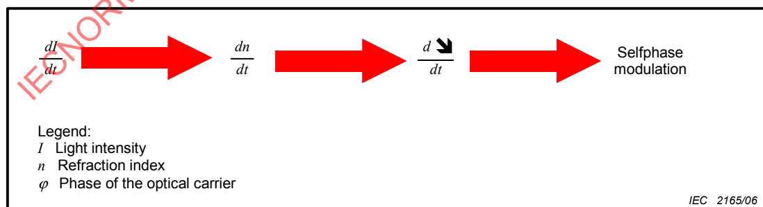
Figure C.6 – Cause of self-phase modulation
