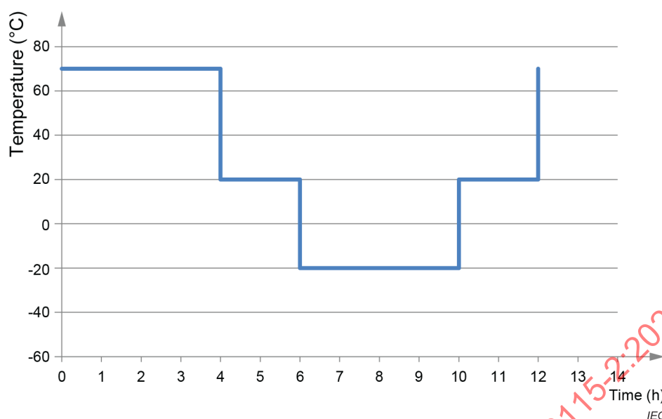
Figure 1 – Temperature profile for 6.4.3 – Temperature cycling test
