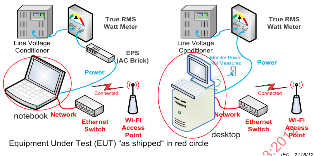
Figure 1 – Typical test setup
