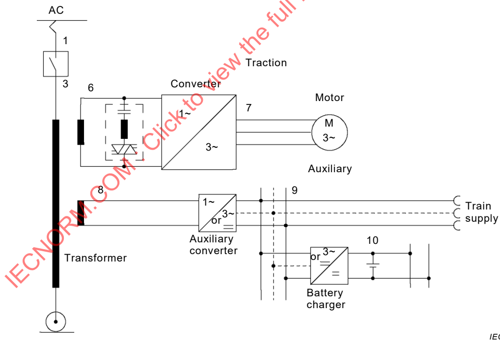
Figure A.2 – AC/AC system with power factor correction filter on the converter side and with DC or three-phase auxiliary and train power supply
