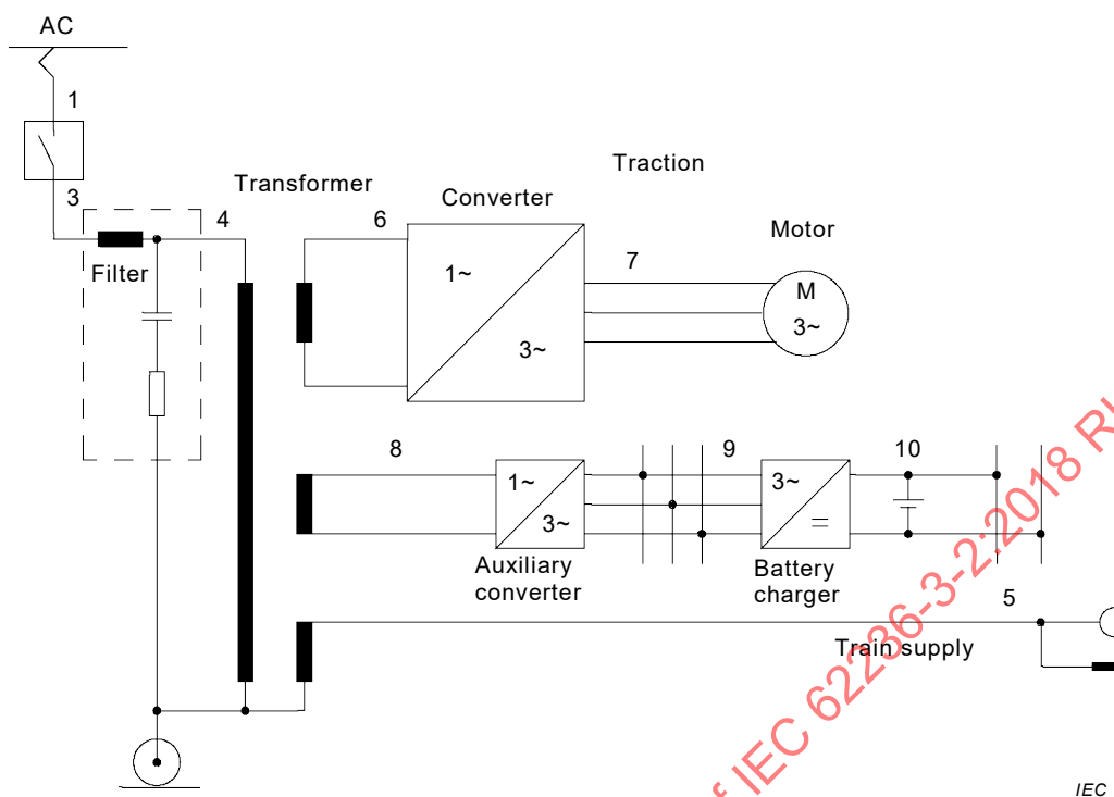
Figure A.1 – AC fed locomotive traction unit with AC traction drive and psophometric filter on the line side
