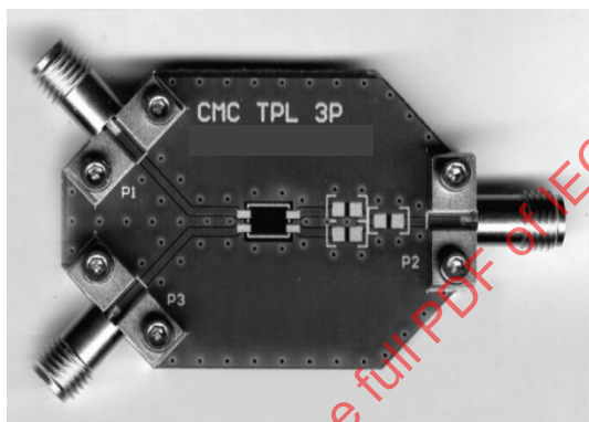
Figure D.7 – Example test board S-parameter measurement – Single ended, top layer
