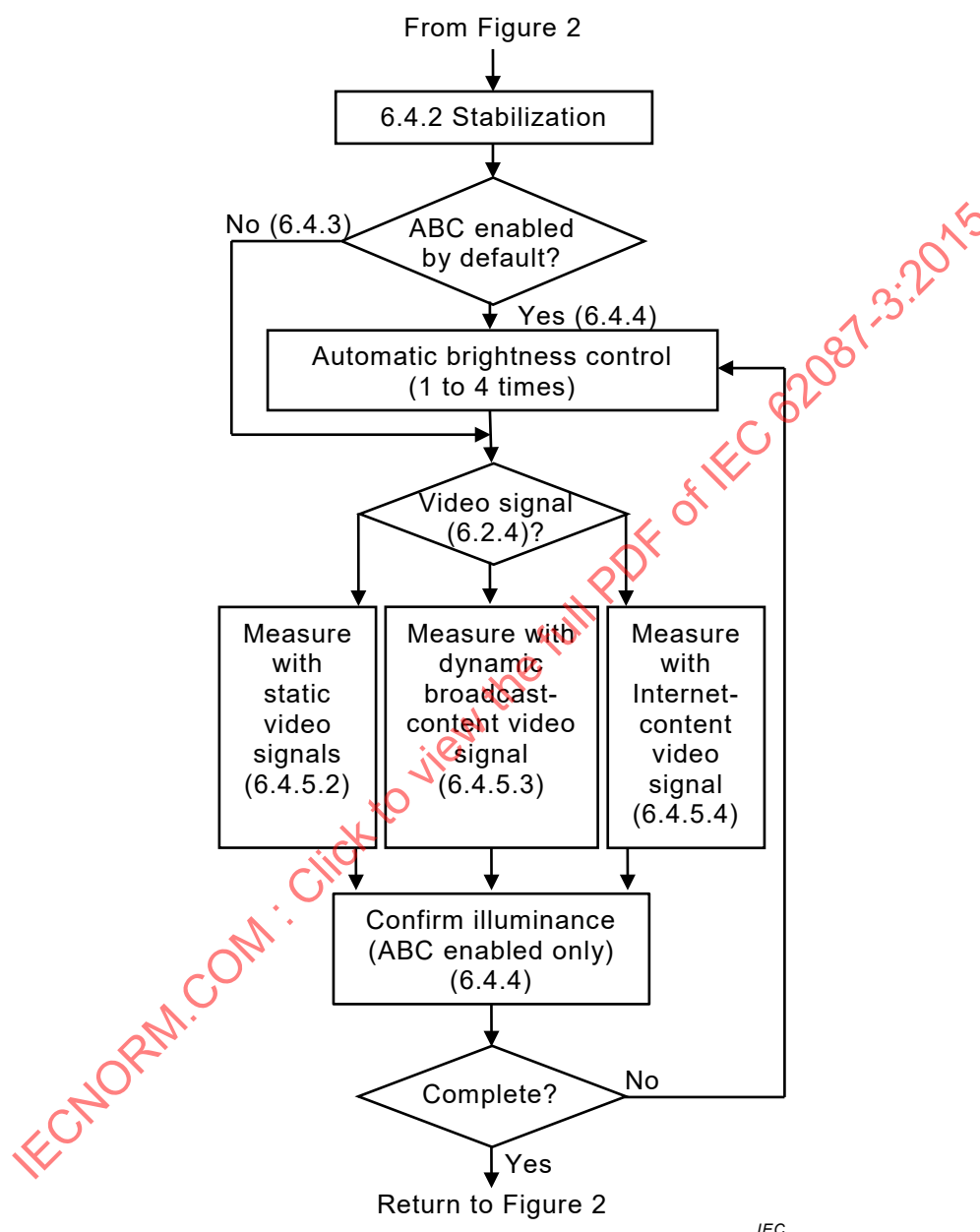
Figure 5 – Order of activities for determining power consumption, On mode
