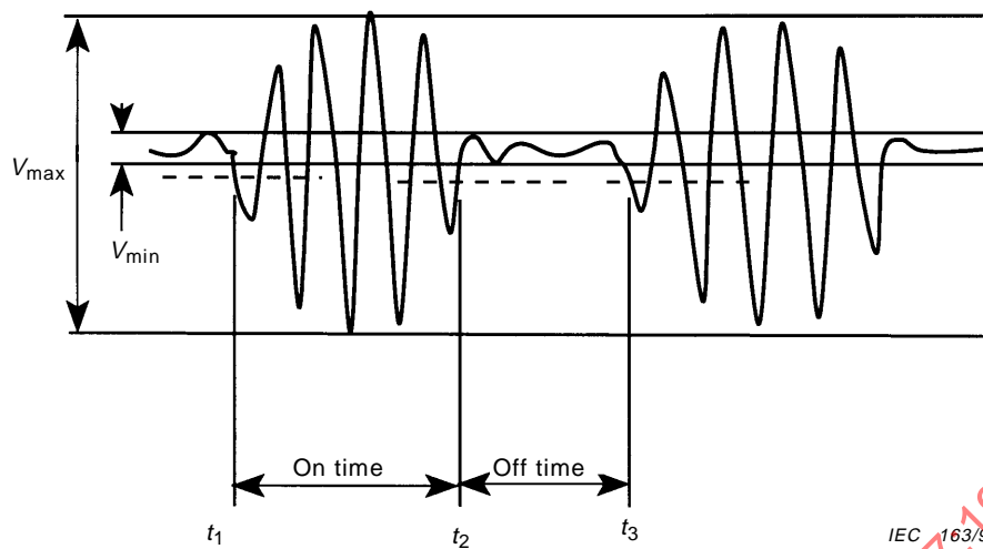
Figure 4 – Illustration of the method of determining duty cycle from an oscilloscope trace. The dotted line is at a level equal to the minimum peak-to-peak level plus 10 % of the difference between the maximum and the minimum peak-to-peak levels
