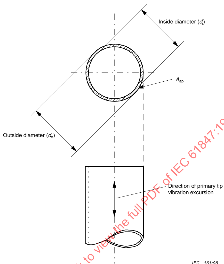
Figure 2 – Example of a primary acoustic output area
