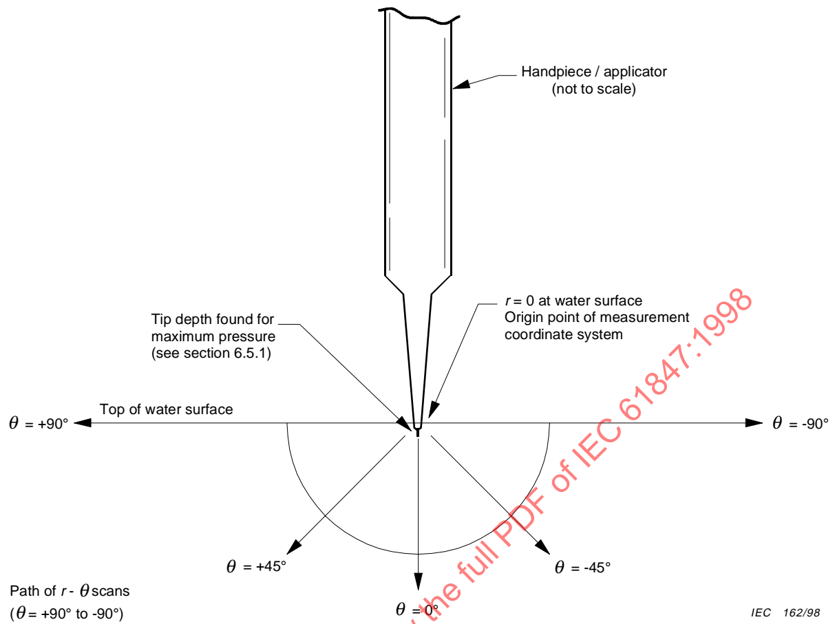
Figure 3 – Measuring the pressure field
