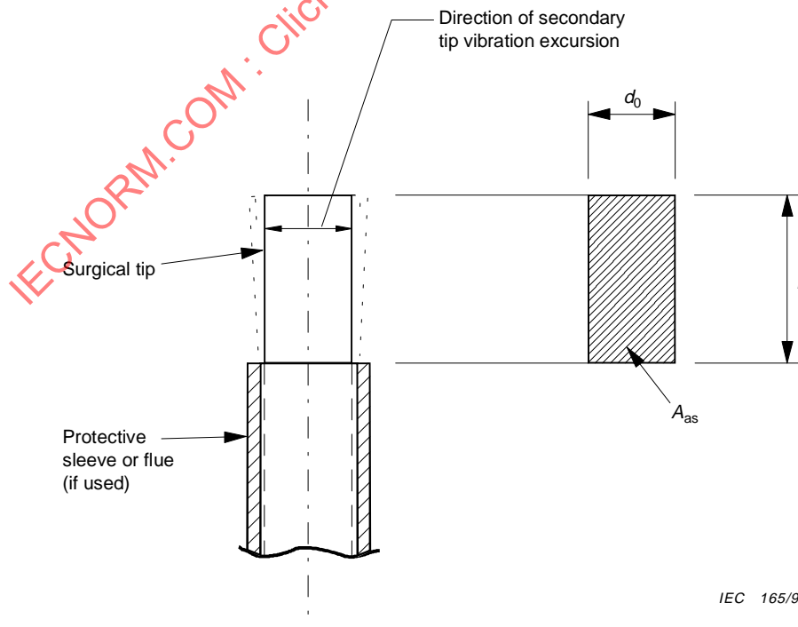
Figure 6 – Example of a secondary acoustic output area
