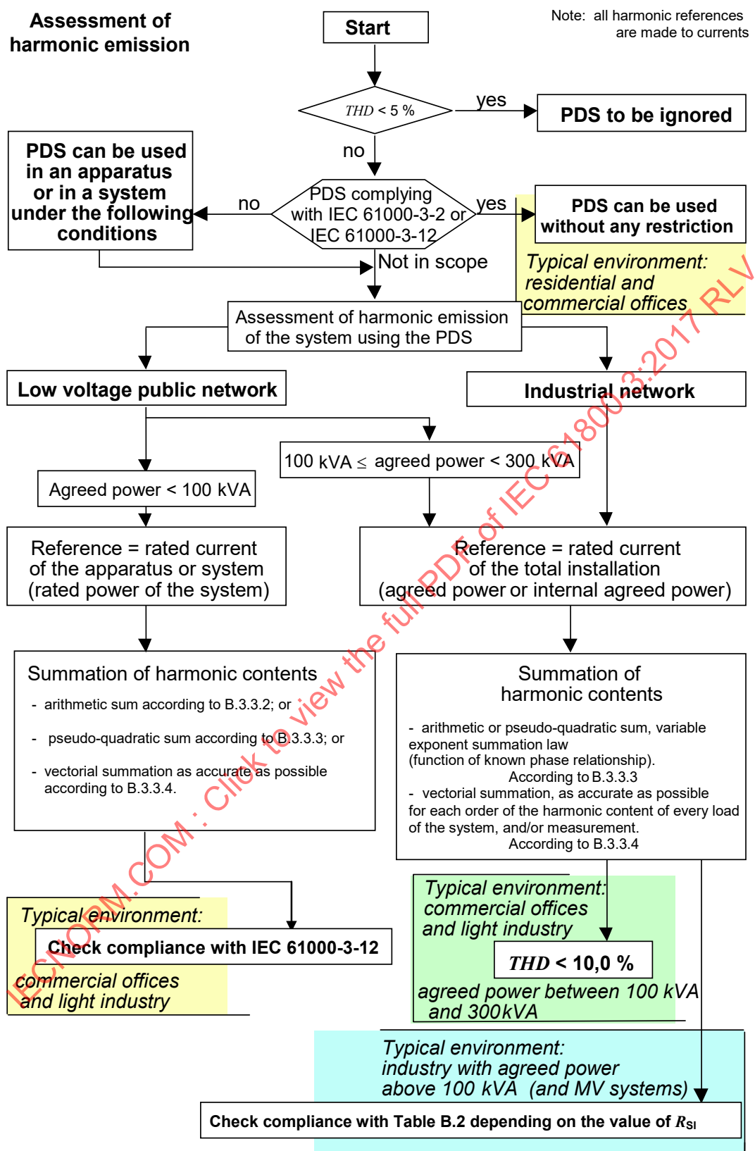
Figure B.8 – Assessment of harmonic emission where PDS is used (apparatus, systems or installations)
