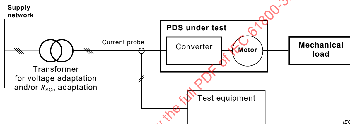
Figure B.5 – Test set-up with mechanical load
