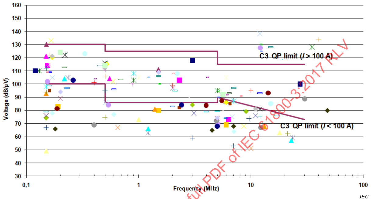
Figure D.1 – Conducted emission of various unfiltered PDSs
