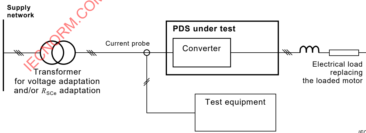
Figure B.6 – Test set-up with electrical load replacing the loaded motor
