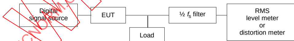
Figure 9 – Circuit arrangement for measuring distortion and noise
