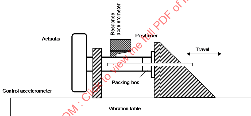
Figure A.1 – Test set-up for vibration test
