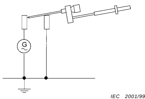
Figure 7c – Disposition du circuit
