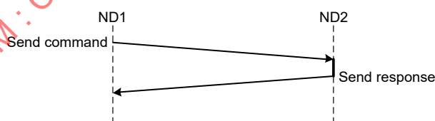
Figure C.1 – Command response communications
