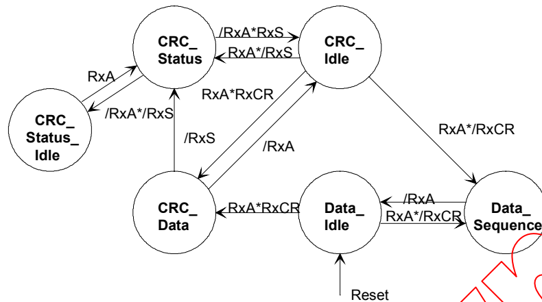
Figure 29 – Protocol machine for the message receipt service
