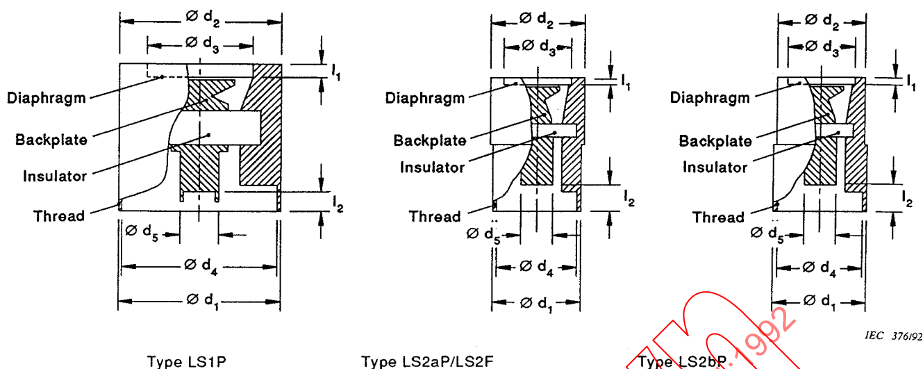
Figure 1 – Mechanical configurations of microphones
